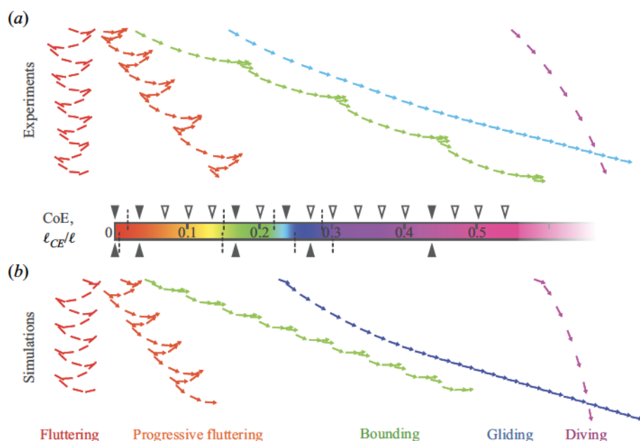
Figure 3. Trajectories of plate wings from experiments in water (a) and simulations (b) and across flight modes attained by varying the (normalized) CoE location \ell_{CE}/\ell . Five distinct modes are observed: fluttering (red), progressive fluttering (orange-yellow), bounding (green), gliding (blue) and diving (purple-magenta). The plates are shown as arrows whose heads indicate the edge towards which the CoM and CoE have been displaced, except in the symmetric case of \ell_{CE}/\ell = 0 (red). Snapshots are shown at rate of 6 per second in all cases. The 17 values of \ell_{CE}/\ell explored in experiments are indicated by the arrowheads above the CoE colour bar, with filled symbols corresponding to the 5 trajectories shown above. Simulations cover \ell_{CE}/\ell finely, and hence we indicate with filled arrowheads below the colour bar only the selected values corresponding to the trajectories below. Dashed lines on the colour bar indicate the critical values of \ell_{CE}/\ell separating the modes.
