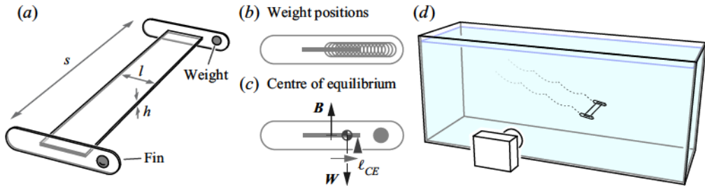
Figure 2. Experiments on the free flight of plates through water. (a) A plate wing and two side fins are laser cut from acrylic plastic, and embedded in the fins are lead weights that serve to displace the CoM. The plate has span length s , chord l and thickness h . (b) Each of 17 flyers is assembled with the paired weights placed symmetrically along the fins at one of the indicated locations. (c) Buoyancy B acting at the centre of volume (CoV) and weight W acting at the CoM lead to a torque balance about the indicated fulcrum or pivot point, which is defined to be the centre of equilibrium (CoE). (d) Each flyer is released within a large water tank, and in-plane or longitudinal motions are recorded with a video camera.
