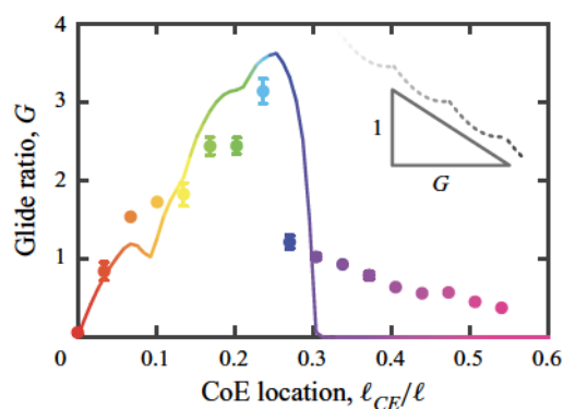
Figure 11. Glide ratio from plate-in-water experiments (markers) and corresponding simulations (curve) across flyers of differing CoE locations. The glide ratio represents forward progress per unit distance of fall during the later stages of flight in which the a terminal behaviour is displayed. The colour coding matches the colour bar for \ell_{CE}/\ell used in previous plots. Gliding (blue tones) tends to maximize G .
