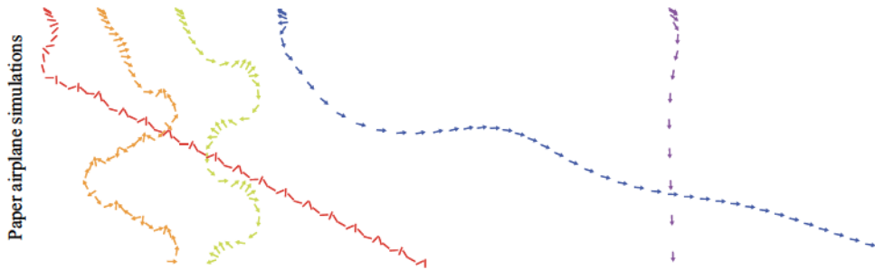
Figure 12. Simulations with parameters relevant to paper airplanes, where the trajectories are coloured according to the map of figure 3. Representative trajectories are shown for \ell_{CE}/\ell = 0, 0.08, 0.14, 0.24 and 0.31 . The simulated motions correspond qualitatively well to the experimental observations of paper airplanes shown in figure 1.
