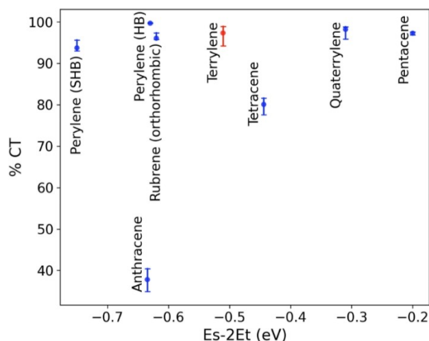
Figure 5. A two-dimensional descriptor for assessing SF candidates. The thermodynamic driving force for SF ( E_s - 2E_t ) is displayed on the x-axis and the singlet exciton charge transfer character (%CT) is displayed on the y-axis. The error bars correspond to the range of %CT values obtained by using different hole positions when performing double-Bader analysis. Terrylene, coloured in red, is compared to other oligoarylene and acene crystals.
