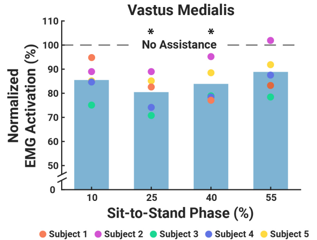
Fig. 3. Muscle activation levels of VM with different assistance peak timings (10%, 25%, 40%, and 55% of the sit-to-stand phase) averaged across 5 subjects. Colored dots represent normalized EMG activation values for each individual, and asterisks indicate statistical significance compared to no assistance ( p < 0.05 ).
