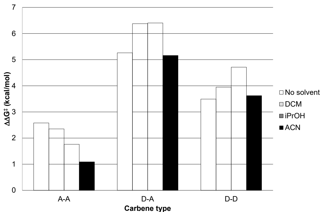
Figure 7. Comparison of the Gibbs free energy barriers difference for insertion of the carbene into the \text{CH}_2 and \text{CH}_3 of propane for acceptor/acceptor (A-A), donor/acceptor (D-A) and donor/donor (D-D) carbenes in gas phase and dichloromethane (DCM), isopropanol ( i\text{PrOH} ) and acetonitrile (ACN) solution.
