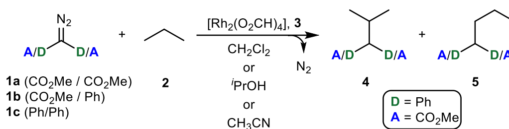
Scheme 2. Rh-catalyzed transformation of A/A, D/A, and D/D diazo compounds and propane to C–H insertion products.
