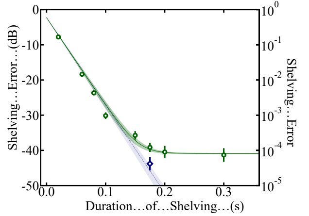
FIG. 4. Error in electron shelving of an ion prepared initially in the {}^2S_{1/2}(F=1) manifold as a function of 411 nm illumination times. The green trace and circles show the error with only the 935 nm light repumping population from the {}^2D_{3/2} states, while the blue trace and diamond shows the error with the 935 nm light replaced by the 861 nm repump scheme. Dashed lines are the theoretical prediction of Eq. (1), with bands indicating the uncertainty in the model due to uncertainty in the {}^2D_{5/2} lifetime and E1-E2 branching ratio. The prediction with the 861 nm repump (blue) is just the second term in Eq. (1).
