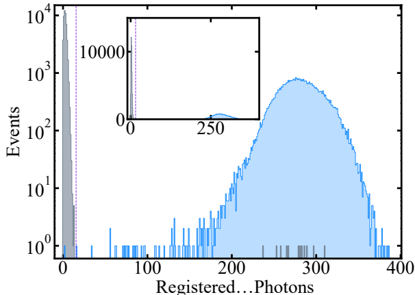
FIG. 2. Fluorescence detection count histograms for attempted SPAM of the |1\rangle (blue) and |0\rangle (gray) ground state hyperfine qubit states in ^{171}\text{Yb}^+ . The inset shows the same data on a linear scale. The predetermined state detection threshold is shown as a dashed purple line, and gives an average SPAM inaccuracy of -39(1) dB.
