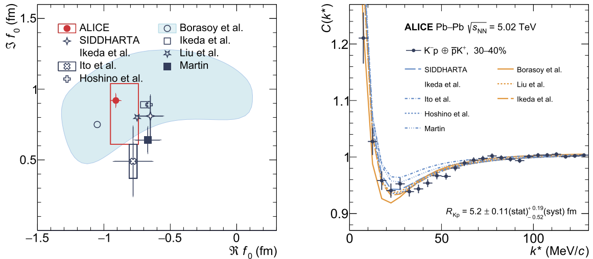
Fig. 3. Left: scattering parameters obtained from the Lednický-Lyuboshitz fit compared with available world data and theoretical calculations. Statistical uncertainties are represented as bars and systematic uncertainties, if provided, as boxes. Right: experimental femtoscopic correlation function for K^-p \oplus K^+\bar{p} pairs in the 30–40% centrality interval, together with various Lednický-Lyuboshitz calculations obtained using the scattering length parameters from Refs. [17,18,75–79] and the source radius from this analysis. The statistical and systematic uncertainties of the measured data points are added in quadrature and shown as vertical bars.
