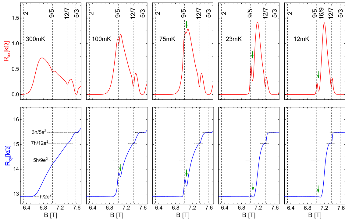
Fig. 2 The dependence on temperature T of the magnetoresistance R_{xx} and Hall resistance R_{xy} of Sample 1 in the range of filling factors 5/3 < \nu < 2 . Labels on vertical dashed lines are filling factors \nu of interest. The electron solid we refer to as the reentrant integer quantum Hall Wigner solid (RIQHWS) is located between filling factors \nu = 9/5 and 16/9 and it is marked by arrows.
