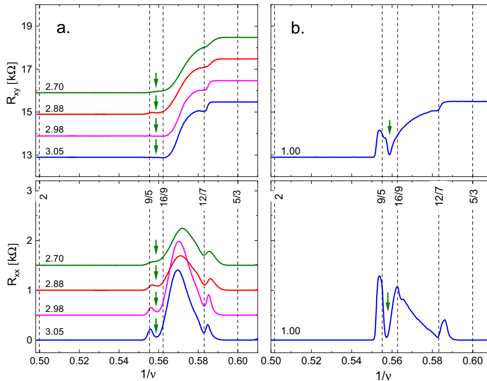
Fig. 3 Reentrant integer quantum Hall Wigner solids in a variable density sample and a sample of fixed density. a Waterfall plots of the magnetoresistance R_{xx} and Hall resistance R_{xy} as plotted against the inverse filling factor 1/\nu of Sample 1 as prepared at different electron densities. Measurements were performed at the temperature of T = 12 mK. b Magnetoresistance R_{xx} and Hall resistance R_{xy} as plotted against the inverse filling factor 1/\nu of Sample 2 of a fixed electron density. This density is significantly lower than that of Sample 1. Measurements were performed at the temperature of T = 5.1 mK. Labels on traces indicate electron densities n in units of 10^{11} \text{ cm}^{-2} . Vertical dashed lines mark locations and values of filling factors \nu of interest and arrows mark the reentrant integer quantum Hall Wigner solid (RIQHS). With the exception of traces at the highest density, traces for Sample 1 are shifted vertically upward for clarity.
