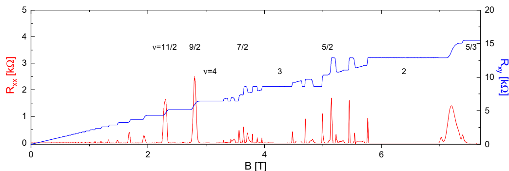
Fig. 1 Magnetoresistance R_{xx} and Hall resistance R_{xy} of Sample 1 over a broad range of magnetic fields B . Traces are obtained at the temperature T = 12 mK. Numerical labels indicate notable Landau level filling factors \nu . Structures of interest develop near B = 7.25 T, in the range of filling factors 5/3 < \nu < 2 .
