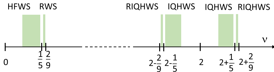
Fig. 4 Schematic diagram of the stability regions of the various Wigner solids in GaAs/AlGaAs system. The Wigner solid we report on is the reentrant integer quantum Hall Wigner solid (RIQHWS), seen between the filling factors \nu = 2 - 1/5 and 2 - 2/9 . The high-field Wigner solid (HFWS) and integer quantum Hall Wigner solid (IQHWS) are related by particle-hole symmetry. Similarly, the reentrant Wigner solid (RWS) and the reentrant integer quantum Hall Wigner solid (RIQHWS) are also related by particle-hole symmetry.
