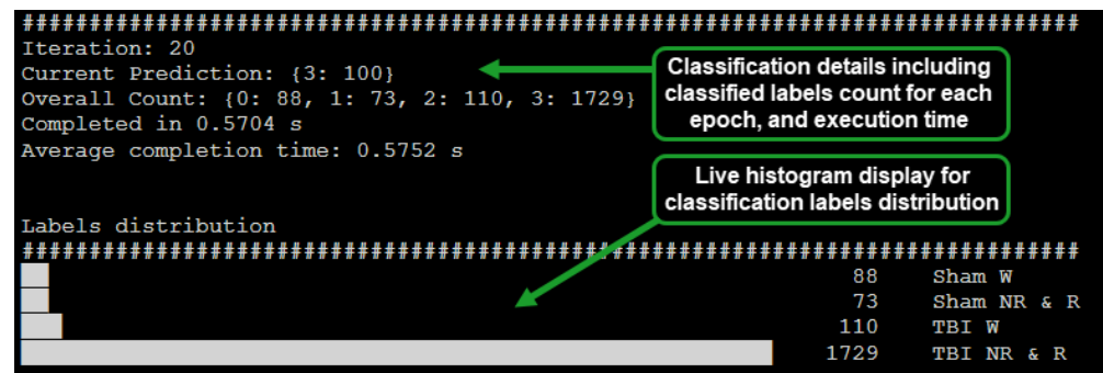
Figure 3. Live classification display for the RPi based system (64 s epoch, batch size: 100).
