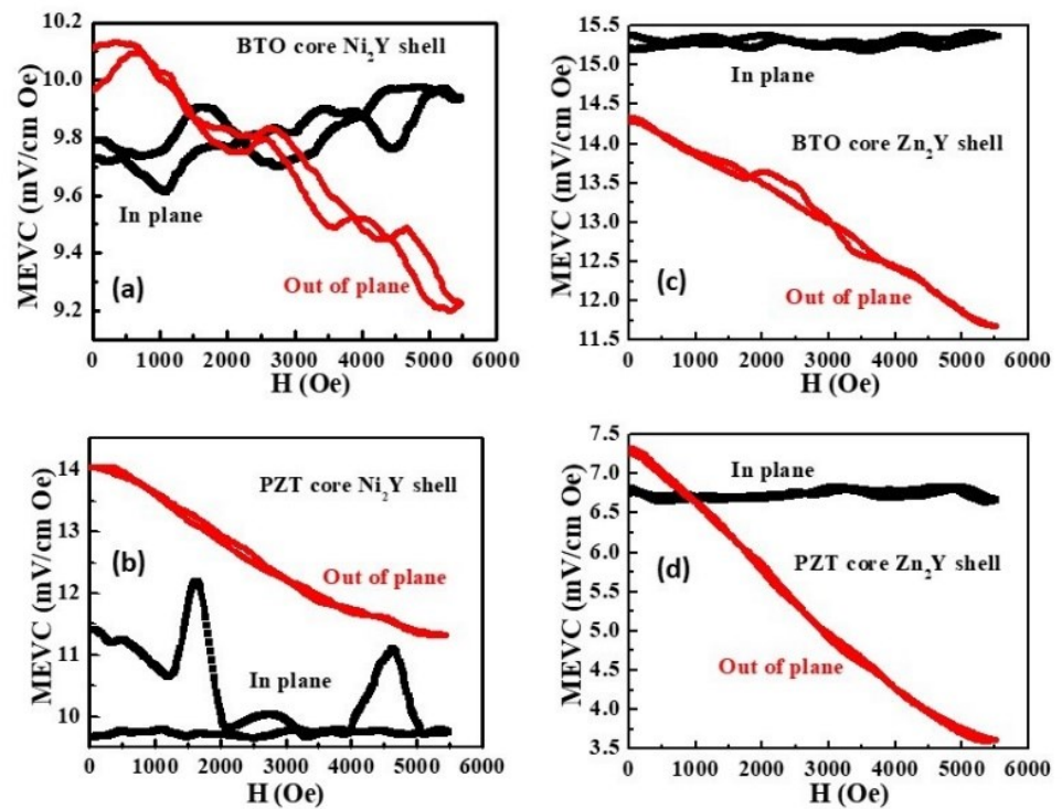
Figure 13. MEVC vs. H data for films of ferroelectric core and shells of Y-type hexaferrites.
