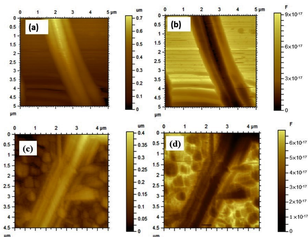
Figure 8. Scanning microwave microscopy (SMM) images recorded at 15.6 GHz showing (a) topography and (b) capacitance for a fiber with a BTO core and Zn 2 Y shell. Similar topography and capacitance images of a fiber with a Zn 2 Y core and PZT shell are shown in (c,d), respectively.
