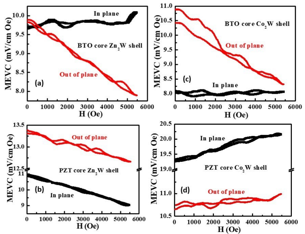
Figure 14. Data as shown in Figure 13 for films of fibers with ferroelectric core and W-type ferrite shells.
