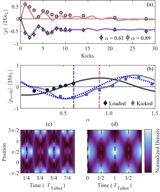
Fig. 3. Initial state dependence of the quantum boomerang effect. All error bars show standard error of the mean on repeated measurements. (a) : Average momentum versus kick number for an initial state consisting of a BEC kicked once by a 60 E_R lattice. Pink circles correspond to \alpha = 0.89 and purple diamonds to \alpha = 0.61 for T = 7 \mu s . Solid lines are predictions of TDSE numerics. (b) : Average momentum after 30 kicks versus \alpha , for an initial condition set by adiabatic loading of a BEC into a 7 E_R lattice (grey circles) and an initial condition set by kicking a BEC once with a 60 E_R lattice (blue squares). Dotted blue line shows infinite-time average momenta predicted by the Floquet diagonal ensemble (Eq. A5). Dashed vertical lines correspond to \alpha values in (a). (c-d) : Calculated density evolution over two Talbot times of a BEC kicked by a 60 E_R lattice (left) and a BEC adiabatically loaded into a 7 E_R lattice which is then quenched off (right). Dashed vertical lines represent time-reversal symmetry axes.
