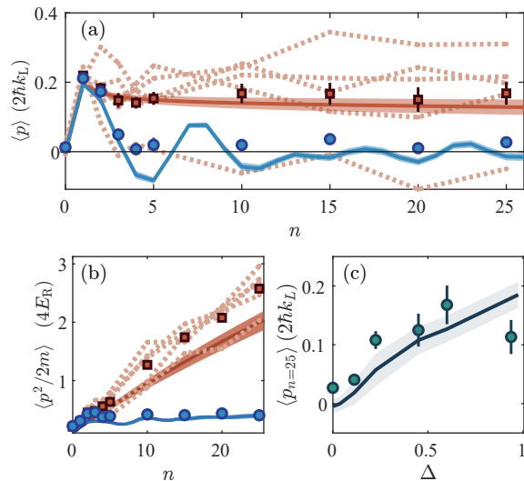
Fig. 4. Destruction of the quantum boomerang effect by stochastic kicking. All error bars correspond to the standard error of the mean for all realizations of randomness. (a): Average momentum measured after n kicks for temporal disorder strength \Delta = 0 (blue circles) and \Delta = 0.6 (red squares). For all data in this figure, T = 8 \mu\text{s} , \alpha = 0.52 , V_0 = 41 E_R , and the initial condition was set by an adiabatic lattice load to 8 E_R . Circles (squares) represent the mean of measurements with 5 separate kick disorder realizations for \Delta = 0 ( \Delta = 0.6 ). Dashed lines show individual realizations. Shaded areas in (a) and (c) show numerically calculated \langle p \rangle \pm \sigma_{\langle p \rangle} with 9000 disorder realizations and 500 initial quasimomenta. The shaded area in (b) includes an additional estimate of the energy accounting for the statistical error in the lattice depth of V_0 = 41 \pm 2 E_R over 500 lattice depths and 500 realizations. (b): Measured mean energy for \Delta = 0 (blue circles) and \Delta = 0.6 (red squares) over 10 points (blue) and 5 disorder realizations (red), illustrating the destruction of dynamical localization by random kicking. (c): Average momentum \langle p \rangle after 25 kicks versus disorder strength \Delta . Dots are averages over 10 disorder realizations, except for \Delta = 0, 0.6 (5 realizations each). The solid line is numerically calculated \langle p \rangle over 9000 disorder realizations, with shaded area showing a one-standard-deviation range.
