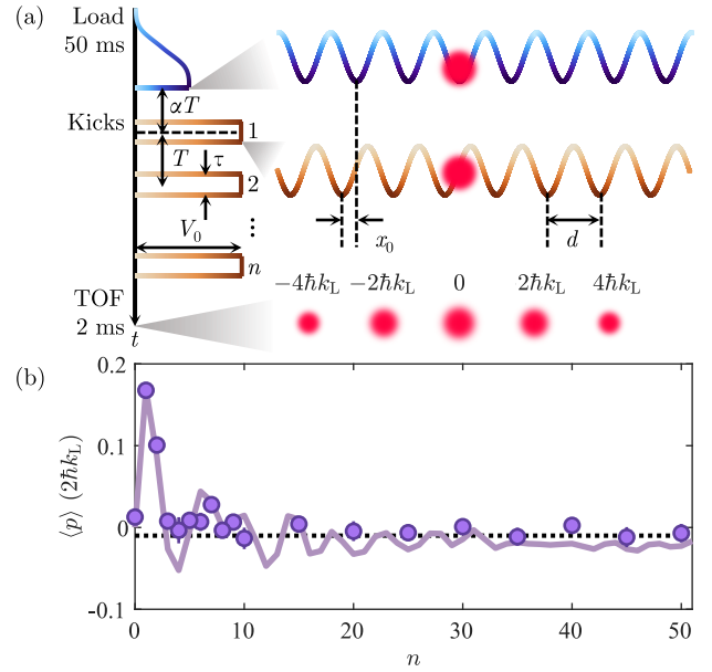
Fig. 1. Observation of the quantum boomerang effect. (a): Experimental sequence. A BEC is loaded into one optical lattice and then kicked with a second, phase-shifted lattice. The momentum distribution is measured after free expansion. BEC size and timeline are not to scale. (b): Measured average momentum versus kick number, for parameters given in the text. The return to the origin demonstrates the quantum boomerang effect. Error bars show standard error of the mean on ten repeated measurements. Solid curve is the numerical prediction. Dotted line represents infinite-time average predicted by the Floquet diagonal ensemble (Eq. A5).
