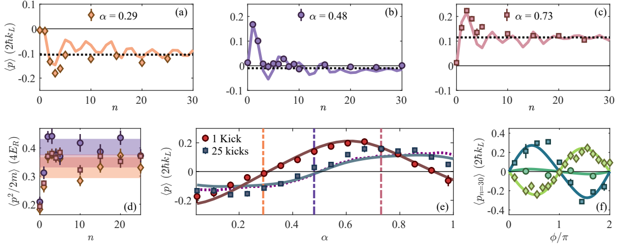
Fig. 2. Characterization of the quantum boomerang effect. All error bars show standard error of the mean on repeated measurements. (a-c) : Average momentum vs. kick number for V_0 = 41 E_R and T = 8 \mu s , at \alpha = 0.29, 0.48 , and 0.73 respectively. Solid curves show numerical predictions. Dotted lines show infinite-time average momenta predicted by the Floquet diagonal ensemble (Eq. A5). \phi = 0.9\pi/2 for all experimental runs. (d) : Measured energy vs. kick number for all three values of \alpha . Shaded areas indicate long-term energy by averaging data points between 10 and 25 kicks. (e) : Measured average momentum after 1 kick (red circles) and 25 kicks (blue squares) vs. \alpha for the same experimental parameters. Same-color solid lines show numerical predictions. Dashed vertical lines indicate \alpha in (a-c). Dotted purple line shows prediction of the Floquet diagonal ensemble [13]. (f) : Average momentum after 30 kicks vs. \phi for V_0 = 70 E_R , T = 7 \mu s , and \alpha = 0.15 (diamonds), 0.48 (circles), and 1.05 (squares).
