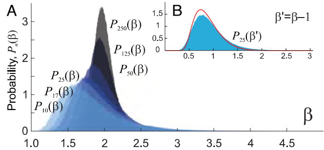
Fig. 10. \beta -distributions. (A) Histograms of \beta -values obtained for 10^6 sequences containing n = 17, 25, 50, 125 , and 250 elements peak in a vicinity of the impartial mean \beta^* and rapidly decay for \beta \lesssim 1.2 and \beta \gtrsim 3.5 . (B) The distribution of \beta' = \beta - 1 for sequences containing about n = 25 points is close to the universal Kolmogorov distribution P(\lambda) (red line, Fig. 2A).
