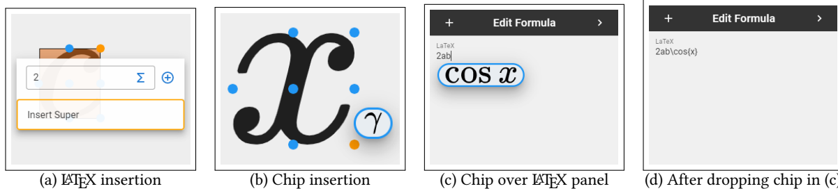
Figure 2: Inserting Formulas. (a) Inserting ‘2’ as an exponent to ‘c’ using a \text{\LaTeX} string. (b) Inserting ‘ \gamma ’ in a chip as subscript of x . (c) A chip containing ‘ \cos x ’ hovering over the \text{\LaTeX} panel (at right in Fig. 1) - the cursor is at the end of the \text{\LaTeX} string. (d) After dropping ‘ \cos x ’ on the canvas, appending ‘ \cos x ’ at the cursor location.
