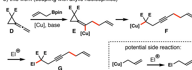
Scheme 1. Approaches for allyl-allene coupling
