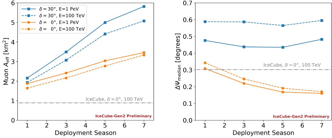
Figure 4: Plots of two metrics of the performance of the detector performance: the muon effective area (left) and the angular resolution (right) as a function of time for several choices of muon energy and declination.
