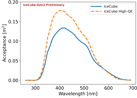
Figure 3: The acceptance to photons as a function of wavelength for two different types of optical modules used in IceCube: the standard IceCube OM, and a high quantum-efficiency variant used in DeepCore.
