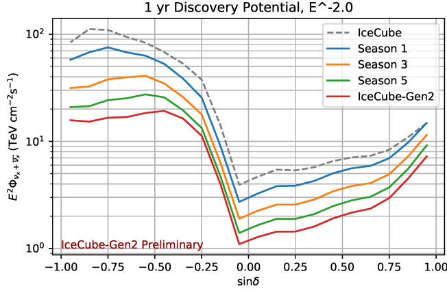
Figure 5: One-year time-integrated discovery potentials for a steady point source of neutrinos with a unbroken power law spectrum E^{-2} . Each line indicates a different year of IceCube-Gen2 construction. Also shown for reference is the 1-year discovery potential of IceCube. We emphasize that one year time-integrated discovery potentials are only shown for purpose of comparison, as the achieved discovery potential in each season will be significantly better if it is combined with the previous years data.
