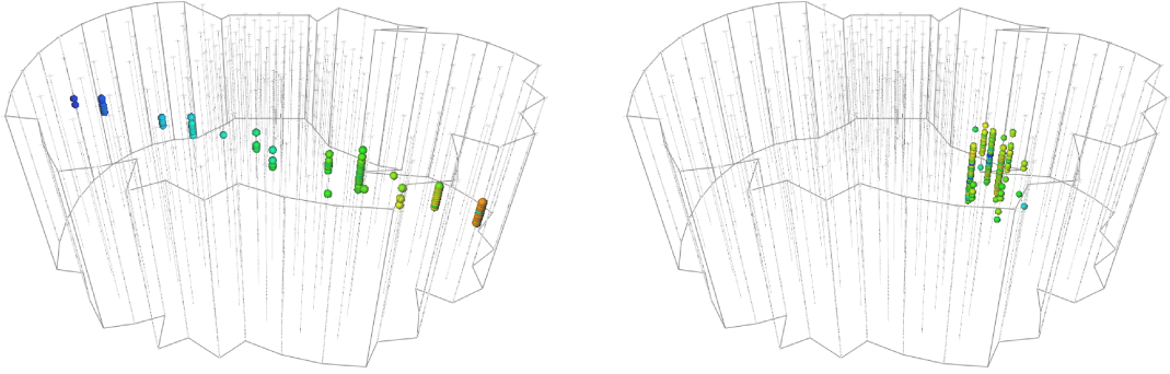
Figure 2: A view of the two main "morphologies" of neutrino interactions expected in the optical component of IceCube-Gen2: "tracks" (left) "cascades" (right). The size of a module is proportional to the quantity of the light recorded, while the color indicates the relative arrival time of the light (with red indicating earlier arrival times, and blue indicating later arrival times).
