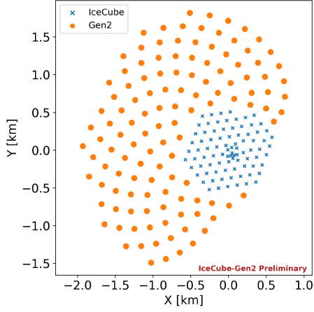
Figure 1: A top-down view of the IceCube-Gen2 optical detector, with the original 86 IceCube strings marked with crosses, and the 120 new Gen2 strings marked with circles.
