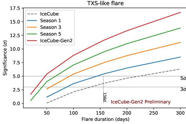
Figure 6: Significance as a function of flare duration for various stages of IceCube-Gen2 construction including trials correction. Backgrounds here are calculated from the previously mentioned atmospheric and prompt fluxes, summed with an additional diffuse E^{-2} astrophysical background component. Vertical bar in the center marks the measured flare duration in IceCube. IceCube significance included for reference.
