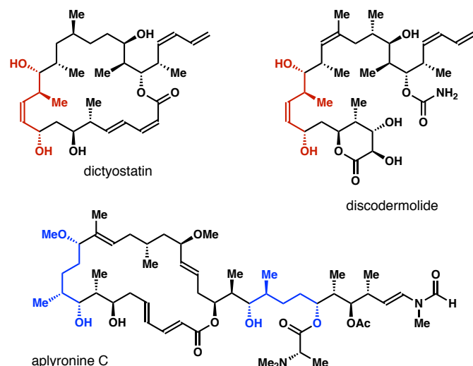
Figure 1. Selected natural products that contain ( Z )-2-methyl-3-pentene-1,5-diols or their reduced forms
