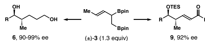
Scheme 1. Approaches to ( Z )-2-methyl-3-pentene-1,5-diols
