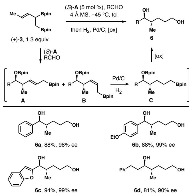
Scheme 3. Enantioconvergent synthesis of diols 6
