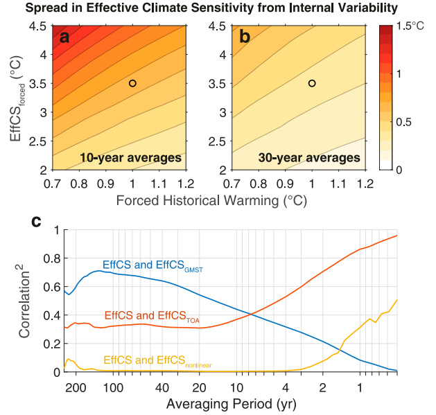
FIG. 10. Two-standard-deviation ( \approx 95\% ) spread in effective climate sensitivity ( \text{EffCS} ) from superimposing internal variability from CMIP6 piControl simulations on an assumed externally forced historical warming ( \bar{T}_{\text{forced}} ; x axis) and a radiative response corresponding to a forced effective climate sensitivity ( \text{EffCS}_{\text{forced}} ; y axis), where \text{EffCS} is calculated from (a) 10-yr running averages and (b) 30-yr running averages of Eq. (6) . Values are the median across 35 CMIP6 models. Black circles show the values of \bar{T}_{\text{forced}} and \text{EffCS}_{\text{forced}} used in Figs. 11 and 12 . (c) Multimodel mean squared correlation between anomalies in \text{EffCS} and its components due to internal variability in GMST and GMTOA, as a function of the averaging period used to compute \text{EffCS} . See the appendix for more details of this decomposition.
