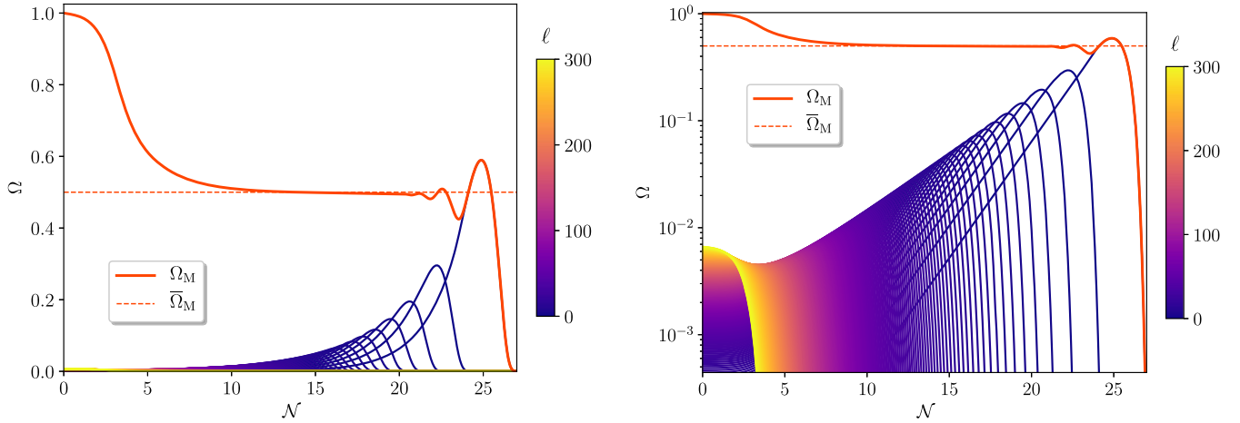
FIG. 2. The individual matter abundances \Omega_\ell (orange and blue) and the corresponding total matter abundance \Omega_M (red), plotted as functions of the number N of e -folds since the initial \phi_\ell production. These curves were generated through a direct numerical solution of the relevant Boltzmann equations for our discrete tower of decaying states without invoking any approximations and correspond to the parameter choices (\alpha, \gamma, \delta) = (1, 7, 1) [for which \bar{\Omega}_M = 1/2 ], with \Delta m = m_0 , N = 300 , and \Gamma_{N-1}/H^{(0)} = 0.01 . In the left panel the abundances are plotted on a linear scale, while in the right panel these same abundances are plotted on a logarithmic scale. We see that our system begins with \Omega_M = 1 at t = t^{(0)} , with each individual \Omega_\ell component exhibiting a nontrivial behavior, first growing as a power law due to cosmological redshifting before ultimately decaying exponentially. Despite this complexity, their sum \Omega_M nevertheless evolves toward a stasis epoch in which \Omega_M remains essentially constant for approximately 15 e -folds before exiting stasis. Even longer periods of stasis can be produced if N is increased. This thereby provides a concrete realization of the basic stasis mechanism sketched in Fig. 1. Eventually the stasis ends as we approach the final decays of the lightest modes.
