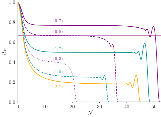
FIG. 4. The total matter abundance \Omega_M , plotted as a function of the number N of e -folds since the initial \phi_\ell production time t^{(0)} for a variety of different benchmark values of (\alpha, \gamma) satisfying the constraints in Eq. (3.19). For each plot we have taken \delta = 1 , \Delta m = m_0 , N = 10^5 , and H^{(0)}/\Gamma_{N-1} = 0.1 as relevant benchmarks. Each curve begins at \Omega_M = 1 at the initial time t^{(0)} and eventually falls to \Omega_M \rightarrow 0 as t \rightarrow \infty . However, we see that in each case there is a prolonged epoch lasting many e -folds during which \Omega_M(t) settles into a stasis state with \Omega_M(t) = \bar{\Omega}_M ; indeed the duration of the stasis state can be increased at will simply by increasing N . For each value of (\alpha, \gamma) , the corresponding stasis values \bar{\Omega}_M are indicated with horizontal dashed lines. Ultimately in each case, the period of stasis ends as we reach the final \phi_\ell decays; the resulting oscillations in \Omega_M reflect the discretization effects associated with the successive final decays.
