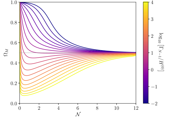
FIG. 5. The total matter abundance \Omega_M , plotted as a function of the number N of e -folds since the initial \phi_\ell production time t^{(0)} for a variety of different values of \Gamma_{N-1}/H^{(0)} , where H^{(0)} is the value of the Hubble parameter at the \phi_\ell production time t^{(0)} . For this plot we have chosen the benchmark values (\alpha, \gamma, \delta) = (1, 7, 1) and taken \Delta m = m_0 and N = 300 . We see that as \Gamma_{N-1}/H^{(0)} increases, our decays occur more rapidly and \Omega_M therefore drops more rapidly from its initial value 1 after t^{(0)} . Indeed, for \Gamma_{N-1}/H^{(0)} \gtrsim 3 , the initial drop in \Omega_M is so rapid that \Omega_M initially drops below the stasis value \bar{\Omega}_M before rebounding due to cosmological expansion; \Omega_M therefore ultimately approaches the stasis value \bar{\Omega}_M from below. Such curves then correspond to trajectories in Fig. 3 for which stasis is approached from the \Omega_M < 1/2 region. However, in all cases our system is inevitably drawn toward the same stasis configuration, illustrating that the stasis state is indeed a global attractor for this system.
