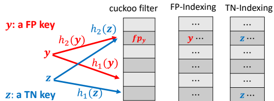
Figure 5: TN-indexing table and FP-indexing table
