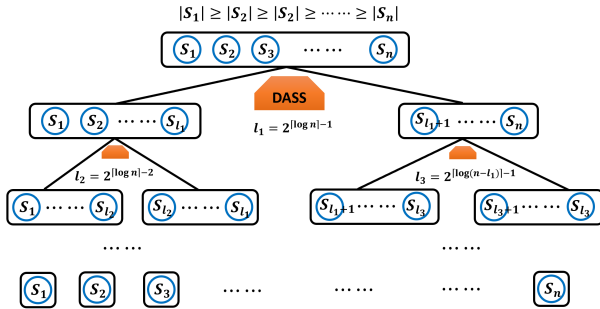
Figure 17: Decision tree of DASS for multi-set query.
