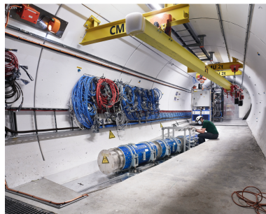
Figure 7: Calorimeter of the FASER main detector
