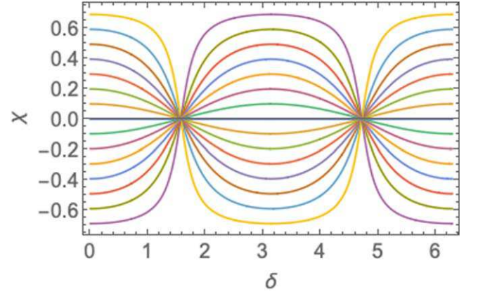
Figure 4. PA \chi of linear polarization as a function of retardance \delta for \chi_0 between 0 and \pi/2 with a step \pi/32 ( \chi_0 = \pi/2 is omitted—this would give a straight line at \chi = \pi/2 ). Values of \chi = 0 correspond to maximal circular polarization V = U_0 and U = 0 .
