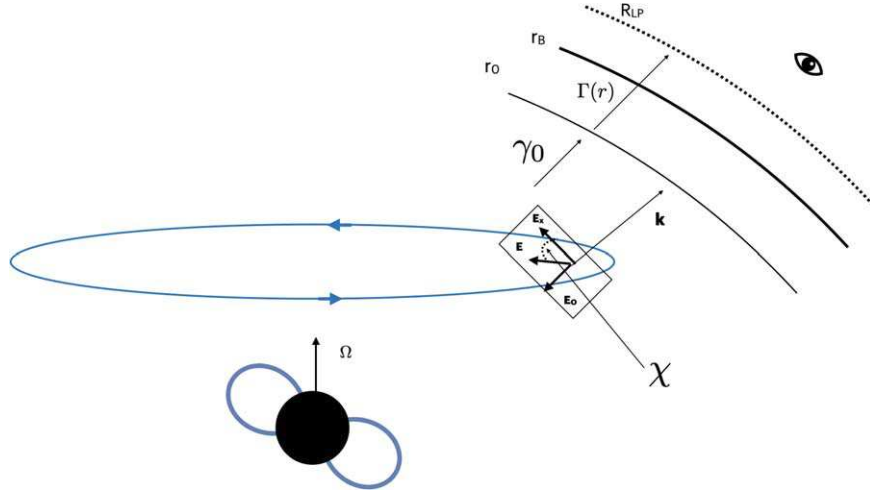
Figure 6. Particle dynamics and polarization in the inner wind. The magnetic field quickly becomes nearly toroidal, and particles stream nearly radially. Until r \sim r_0 = \gamma_0 , the Lorentz factor is the injection Lorentz factor, determined by magnetospheric processes; at larger radii the wind accelerates linearly. Radiation produced in the magnetosphere can be separated into X and O modes. The linear component of polarization makes an angle \chi with respect to the projection of the spin of the neutron star on the sky.
