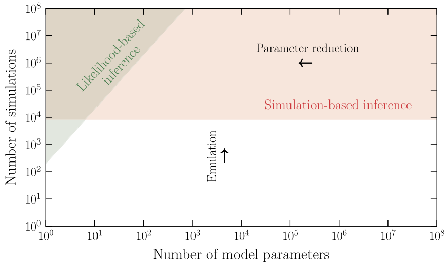
Fig. 4. Simplified comparison of likelihood-based and simulation-based algorithms in the space of number of required/affordable simulations vs. number of model parameters (including parameters of interests, uncertain parameters, and random states of the simulator). In general, the simulation requirements of likelihood-based techniques grow significantly with the number of model parameters. Instead, simulation-based inference techniques can—in principle—directly focus on estimating marginal posteriors for parameters of interest, independently of the total number of parameters. This reduces the need for parameter reduction techniques and enables the comparison of complex simulation results with complex data.
