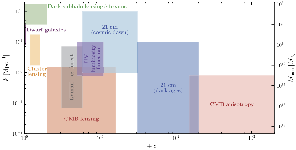
Fig. 3. Schematic representation of the coverage of current and future probes of dark matter physics across various ranges of redshift z (i.e., eras that observable photons or signals primarily originate from), wave number k , and the corresponding halo mass M_{\text{halo}} . The ranges of individual probes are approximate. Note that some of the listed probes are well-established observationally, while some are still in nascent phases of observational development, but they all represent complementary probes of dark matter. We do not include probes that only affect background evolution and thus do not have an associated scale k to display in this figure. Similar figures can be found in (e.g. Buckley and Peter, 2018; Gluscevic et al., 2019; Sabti et al., 2021).
