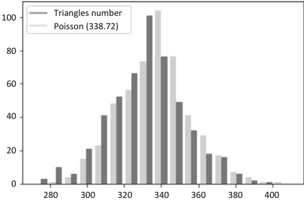
Fig. 1 Histogram of the number of triangles in GRG with 2000 vertices. The distribution of vertex weights W_i \sim Uni(10, 15) , for all i \leq 2000 . The number of realizations is 500
