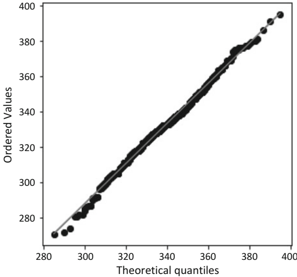
Fig. 2 Q-Q plot for the number of triangles in GRG with 2000 vertices and the Poisson variable Pois(338.72) . W_i \sim Uni(10, 15) , for all i \leq 2000 . The number of realizations is 500
