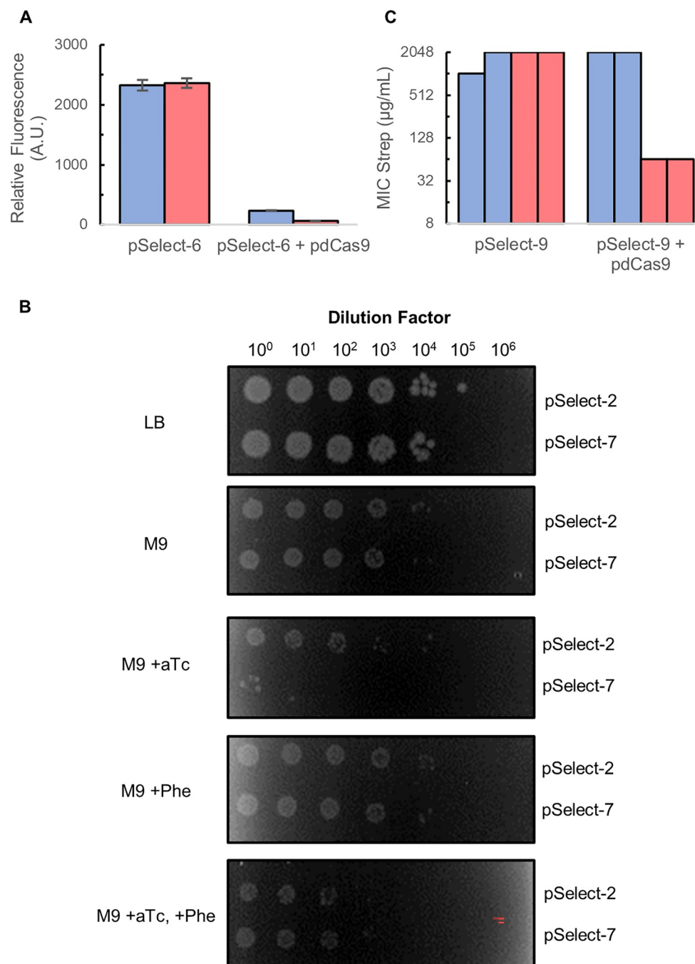
Fig 2. Negative selection system for dCas9 activity. (A) Relative GFP fluorescence after six hours of growth of MG1655 nfsA::(mRFP, sfGFP, Kan R ) cells [3]. Each experiment was performed in the absence (left bars) and presence (right bars) of the pdCas9 plasmid and in the absence (blue bars) and presence (red bars) 2 nM aTc. Error bars represent the standard deviation ( n = 3 ). (B) MG1655 cells spotted on LB-agar and M9-agar. The media along with any supplements it contained is indicated along the column to the left of the plates. aTc was added to a concentration of 2 nM, and phenylalanine was added to a concentration of 10 μg/mL. The selection plasmid present is indicated along the column to the right side of the plates and the dilution factor of each spot is indicated above the plates. (C) Replica minimum inhibitory concentration assays. Each assay was performed twice. Each experiment was performed in the absence (left bars) and presence (right bars) of the pdCas9 plasmid and in the absence (blue bars) and presence (red bars) 2 nM aTc.
