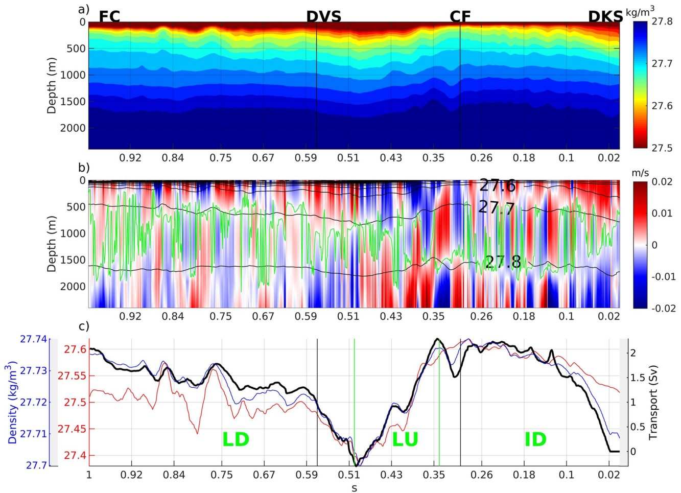
Figure 3. (a) Optimal interpolation-derived multiproduct density ( \sigma_0 ) field along isobath 2400 m. (b) The cross-shore geostrophic velocity field along isobath 2400 m. The positive (negative) values indicate inshore (offshore) flows. The green line indicates the depth at which the maximum (accumulated) vertical transport is found (i.e., levels of no motion). The \sigma_0 = 27.6, 27.7, 27.8 \text{ kg m}^{-3} isopycnals are contoured in black. (c) The density along the boundary from s = 0 to s = 1 averaged in the upper layer (1–300 m, red curve) and the intermediate layer (301–1500 m, blue curve). The maximum vertical transport (black curve) accumulated along the boundary from s = 0 to s = 1 . The upward slopes indicate the downwelling (LD-Labrador Downwelling, s = 0.5 –1, ID-Irminger Downwelling, s = 0 –0.33), and the downward slope indicates upwelling (LU-Labrador Upwelling, s = 0.33 –0.5).
