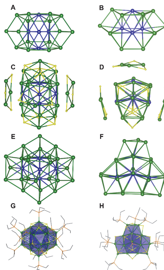
Fig. 1 Solid-state structure of [Ni 30 S 16 (PET 3 ) 11 ]·Et 2 O ( 1 ·Et 2 O) from two different orientations. (A–B) Ni 21 core. (C–D) The three [ cyclo –{Ni(μ-S)} 3 ] units attached to the Ni 21 S 7 core. (E–F) Ni-only structure of 1 . (G–H) Full molecular structure. Color scheme: Ni shell , green; Ni core , blue; S, yellow; P, orange; C, grey. Carbon atoms are shown in wireframe. Diethyl ether solvate molecule and hydrogen atoms were omitted for clarity.
