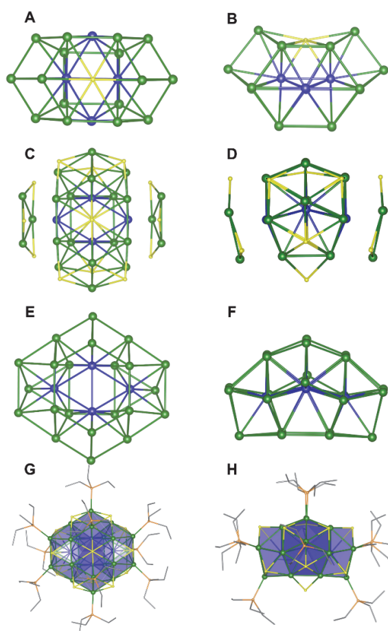
Fig. 3 Solid-state structure of [\text{Ni}_{26}\text{S}_{14}(\text{PEt}_3)_{10}]\cdot\text{C}_5\text{H}_{12} ( \mathbf{2}\cdot\text{C}_5\text{H}_{12} ) from two different orientations. (A–B) \text{Ni}_{26}\text{S}_{14} core. (C–D) The two [ cyclo -{Ni( \mu -S)} 3 ] units attached to the \text{Ni}_{26}\text{S}_{14} core. (E–F) Ni-only structure of 2 . (G–H) Full molecular structure. Color scheme: Ni shell , green; Ni core , blue; S, yellow; P, orange; C, grey. Carbon atoms are shown in wireframe. Pentane solvate molecule and hydrogen atoms were omitted for clarity.
