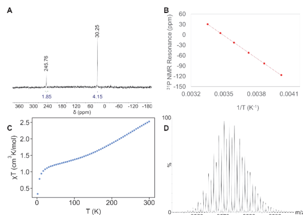
Fig. 2 Characterization data for 1 . (A) Partial 31 P{ 1 H} NMR spectra of 1 in toluene- d 8 . (B) A plot of 31 P{ 1 H} NMR chemical shift versus T –1 for the 30 ppm (25 °C) resonance. (C) Variable temperature magnetic susceptibility (χT) for 1 collected at 10,000 Oe. (D) Partial ESI-MS mass spectrum of 1 in THF (capillary voltage of 2.50 kV, positive ion mode) showing a peak at 3572.43 m/z assignable to [Ni 30 S 16 (PEt 3 ) 11 ] + (calcd 3572.57 m/z ).
