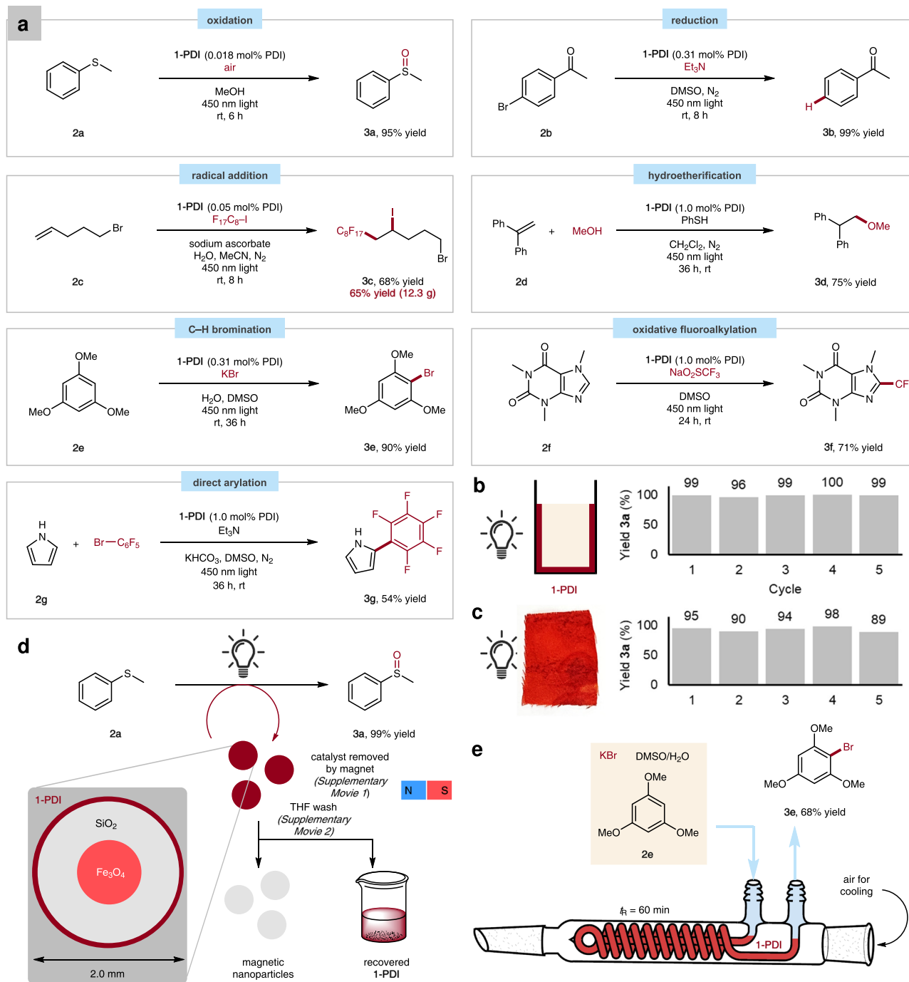
Fig. 3 Synthetic applications of porous-polymer photocatalyst. a Performance of 1-PDI across various reaction classes. b Recyclable usage of 1-PDI as a coating on a glass vial in the photo-oxidation of 2a. c Recyclable usage of 1-PDI deposited on cotton in the photo-oxidation of 2a. d Coated superparamagnetic silica nanoparticles. e Continuous-flow synthesis using a film of 1-PDI in glass tubing.
