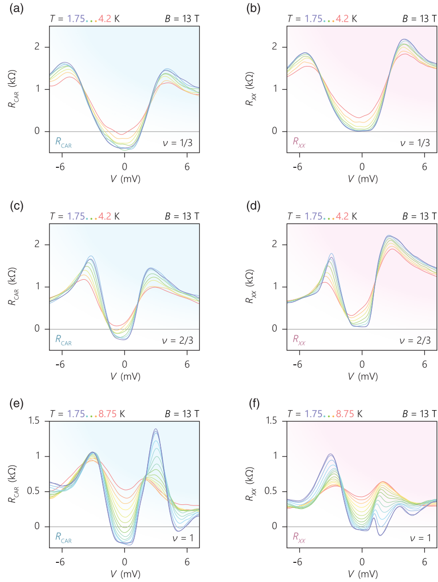
FIG. 11. Transport spectroscopy in device 2 (part 1). (a)–(f) R_{\text{CAR}} and R_{\text{XX}} at several fillings as a function of the incoming edge mode potential V (excitation) for different temperatures T . Crossed Andreev reflection ( R_{\text{CAR}} < 0 ) is limited to below |eV| \sim 1 meV. Increasing excitation and T suppress CAR by increasing bulk conductance for these fillings in this device. The features in (e) and (f) appearing at V \sim 1 mV correspond to the magnon excitation [45,46], missing in other integer and fractional quantum Hall states.
