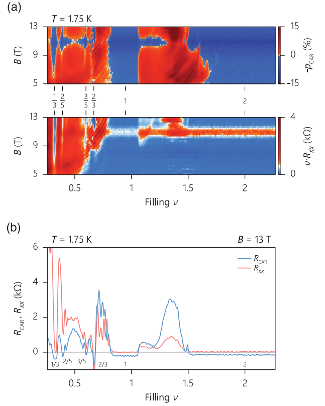
FIG. 10. Magnetic field dependence in device 2. (a) p_{\text{CAR}} and R_{\text{XX}} (normalized for different \nu ) as a function of filling and magnetic field B . Crossed Andreev reflection ( R_{\text{CAR}} < 0 ) is seen for all well-developed \nu . Bulk conduction suppresses CAR observed for lower values of B or for fractional \nu with smaller excitation gaps. (b) R_{\text{CAR}} and R_{\text{XX}} at B = 13 T from (a). Bulk conductance ( R_{\text{XX}} ) is negligible for all highlighted fillings except \nu = 2/3 , a complication related to equilibration in the contact, which is limited to this measurement.
