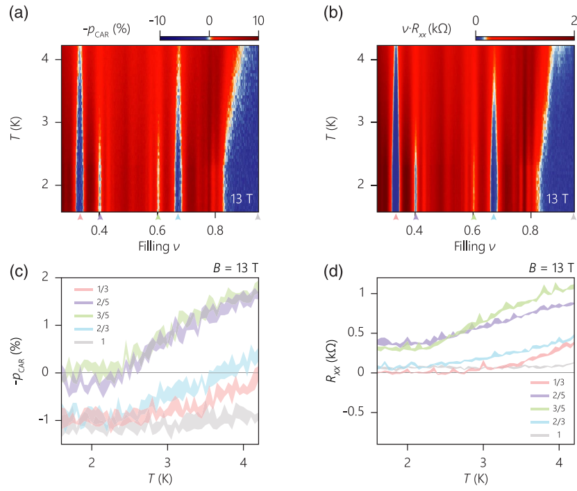
FIG. 13. Temperature dependence in device 2 (part 1, fractional fillings). (a),(b) p_{\text{CAR}} and R_{xx} (normalized for different \nu ) as a function of filling for varying T . Crossed Andreev reflection ( p_{\text{CAR}} > 0 ) is seen for the well-developed fillings \nu = 1/3, 2/3 , and 1, as well as the fillings with smaller excitation gaps \nu = 2/5 and 3/5 , all highlighted with arrows. (c),(d) Vertical cuts, respectively, from (a) and (b). The shades represent the standard deviation.
