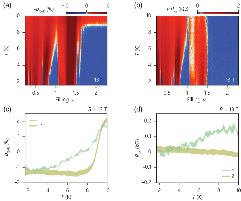
FIG. 14. Temperature dependence in device 2 (part 2, integer fillings). (a),(b) p_{\text{CAR}} and R_{xx} (normalized for different \nu ) as a function of filling for varying T . Crossed Andreev reflection ( p_{\text{CAR}} > 0 ) is seen for both integer fillings \nu = 1 and 2. (c),(d) Vertical cuts, respectively, from (a) and (b). The shades represent the standard deviation. Crossed Andreev reflection at \nu = 2 is undisturbed by bulk conductance and suppressed when the NbN superconductor turns normal at T \sim 9 K.
