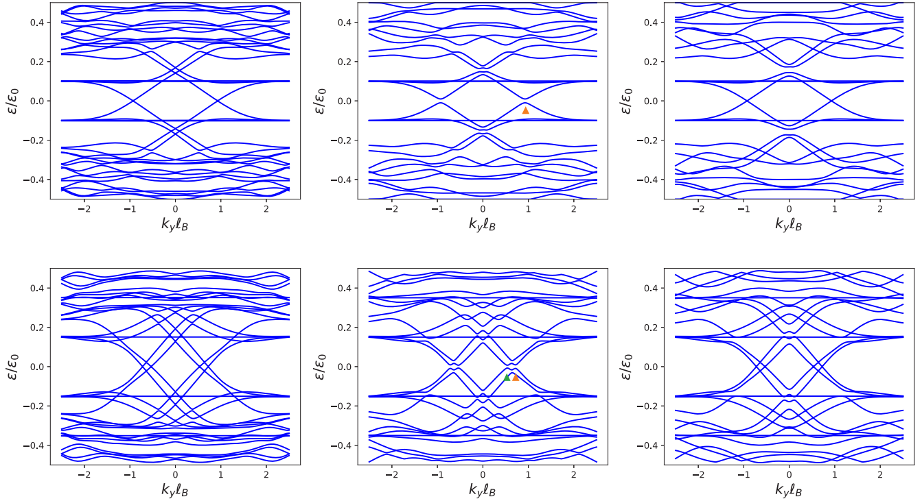
FIG. 17. Bogoliubov spectrum. Top row: \nu = 1 with \mu_n = 0.3\varepsilon_0 . Bottom row: \nu = 2 with \mu_n = 0.55\varepsilon_0 (see the right-hand panel of Fig. S4 in Supplemental Material for the location of the chemical potential [35]). Left-hand column represents the case of a thick superconductor W_s = 15l_B = 10\xi_0 . Middle and right-hand column correspond to a thin superconductor W_s = 6l_B = 4\xi_0 . There is no energy gap in the thick regime, while there is a gap opening in the thin regime when spin-orbit coupling is present (middle column). For reference, we provide the right-hand column which has no spin-orbit coupling. In the other panels we set \lambda_{Rx} = \varepsilon_0 . It is evident that either turning off the spin-orbit coupling or making the superconductor thick prevents the edge modes from hybridizing and leads to a gapless spectrum with propagating Andreev edge states along the QH-superconductor interface. For these simulations, the system parameters are set as follows: \Delta_1 = 0.5\varepsilon_0 , \Delta_2 = 0.6\varepsilon_0 , m_s = 3\varepsilon_0 , \mu_s = 8\varepsilon_0 , \lambda_{Ry} = \lambda_{SO} = 0 , \lambda_{Rx} = \varepsilon_0 .
