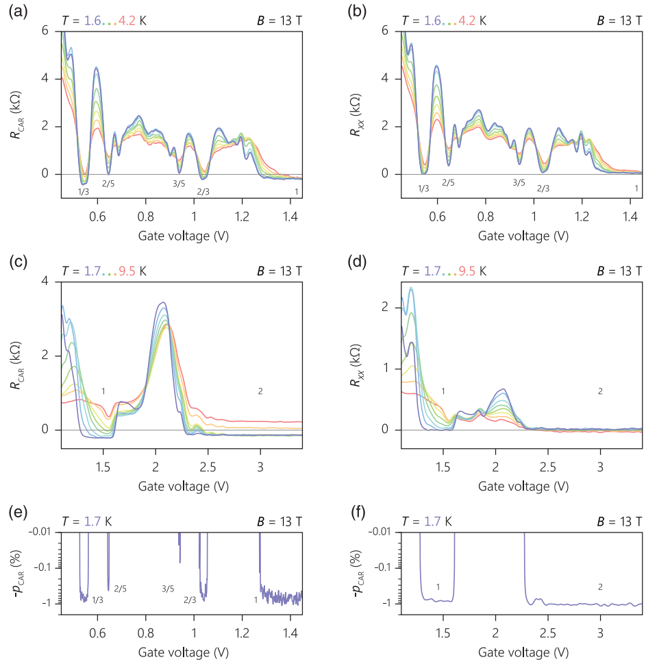
FIG. 8. Crossed Andreev reflection in the FQH state in device 2. (a),(b) R_{\text{CAR}} and R_{\text{XX}} as a function of gate voltage at B = 13 T for different temperatures T . R_{\text{CAR}} < 0 at the highlighted fillings indicates crossed Andreev reflection. (c),(d) Same as (a) and (b) but for integer fillings 1 and 2 in a larger T range. (e),(f) p_{\text{CAR}} at T = 1.7 K, respectively, from (a) and (c).
