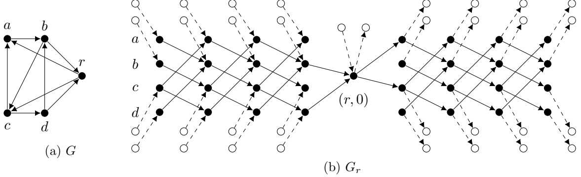
Figure 1: Construction of G_r given G = (V, E) and r \in V
