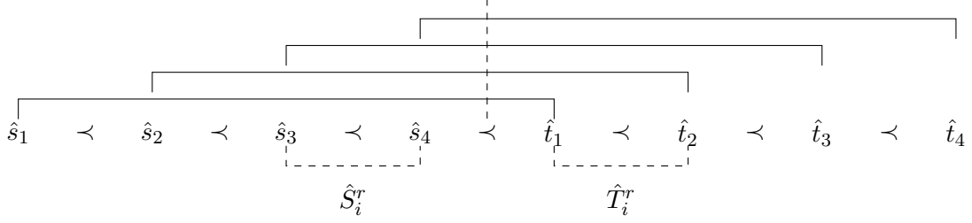
(a) The original path selection by LP (5)
