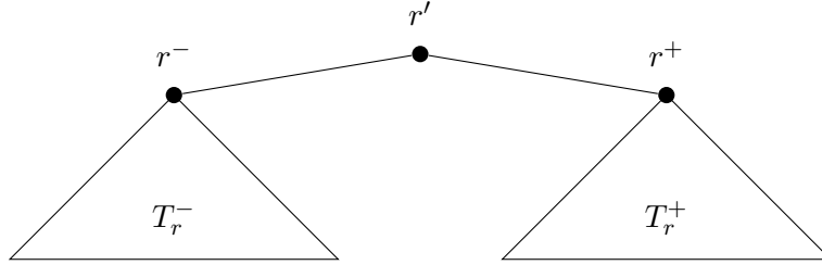
Figure 2: Construction of H_r
