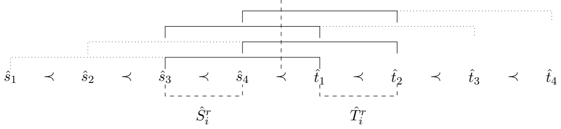
(b) The adjusted path selection with representative endpoints for LP (5)
