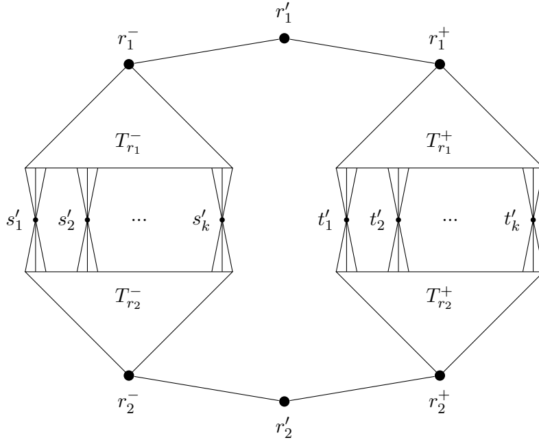
Figure 3: Construction of H'
