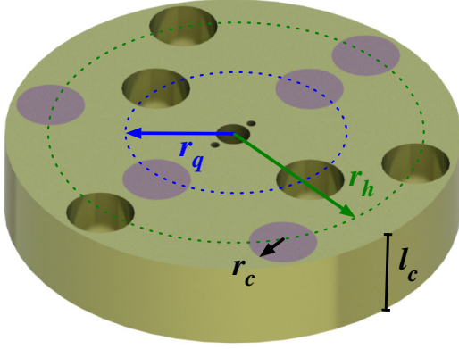
FIG. 2. CAD rendering of the NCal rotor. Solid (purple) regions indicate the holes filled with tungsten cylinders and gold regions indicating the aluminum disk and the unfilled cylindrically shaped holes. Geometrical parameters of the rotor are also highlighted for clarity.
