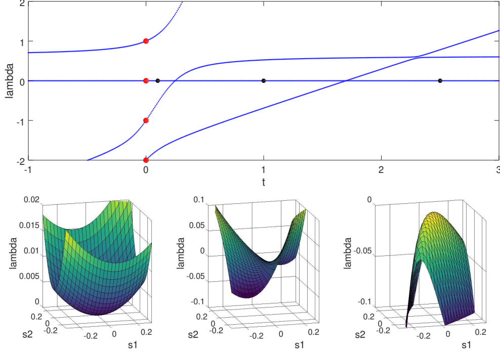
FIGURE 1. Top: the eigenvalues of H(t, \vec{0}) as functions of t ; red (larger) dots highlight the eigenvalues of H(0, \vec{0}) , black (smaller) dots indicate the values of t where the lateral variation is explored in the bottom figures. Bottom: the continuation of the eigenvalue 0 in the spectrum of H(0.1, \vec{s}) , H(1, \vec{s}) and H(2.5, \vec{s}) , correspondingly, shown as functions of \vec{s} = (s_1, s_2) .
