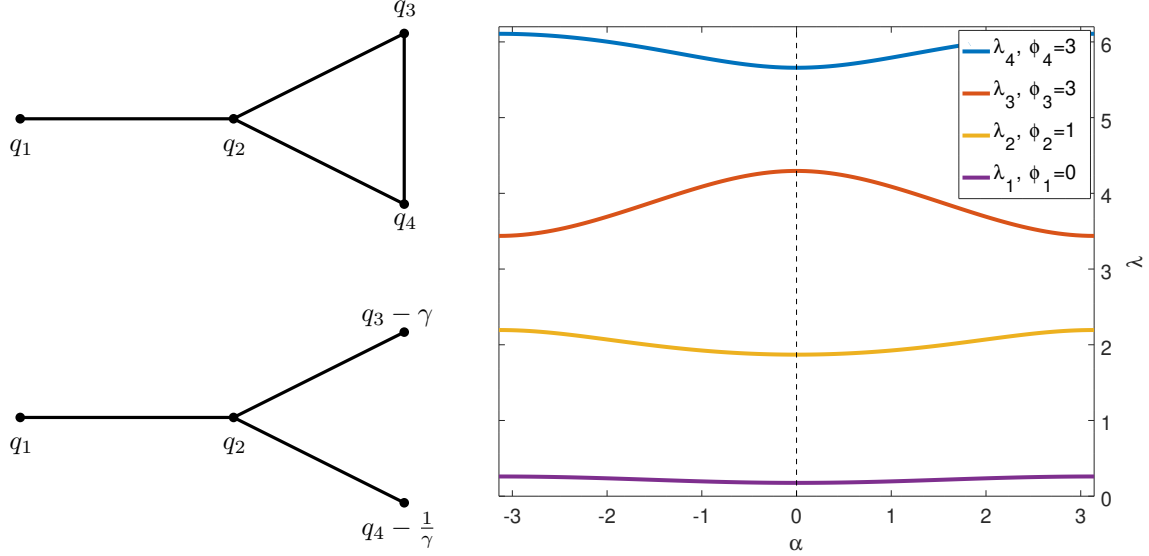
FIGURE 2. Top left: the graph corresponding to operator H in Example 4.1. Bottom left: the graph corresponding to operator S . Right: eigenvalues of the matrix H(\alpha) as function of \alpha \in [-\pi, \pi] ; the legend lists the “sign flip counts” for the corresponding eigenfunction of H(0) . We used q_1 = 1 , q_2 = 2 , q_3 = 4 and q_4 = 5 .
