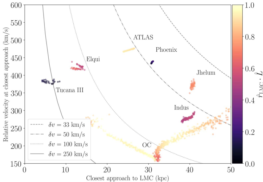
Figure 3. Predicted perturbation by the LMC on each stream. The x-axis shows the distance of closest approach, and the y-axis is the relative velocity at closest approach. For each stream, we plot points spaced by 0^\circ 1 in \phi_1 . The curves represent lines of constant perturbation, assuming the interaction is impulsive. The color represents the component of the velocity kick in the direction of the angular momentum vector. Kicks in this direction present as offsets between the stream track and the proper motion direction, which are most easily measurable given currently available data.
