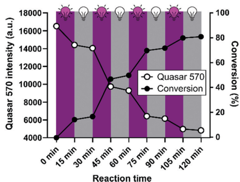
Fig. 3 Temporal control in SP-CuAAC, reaction conditions: [Q570-DNA]/[IN 3 -Cy5]/[CuSO 4 ]/[THPTA]/[SP]: 1/1.1/2.5/12.5/1000, [Q570-DNA] = 0.1 mM, in PBS with 3.7% DMSO at r.t., under UV light (6 mW cm -2 ) in an ambient atmosphere. The conversion was calculated using the F/F_0 of Q570 and the linear regression equation from Fig. S6A (ESI†).
