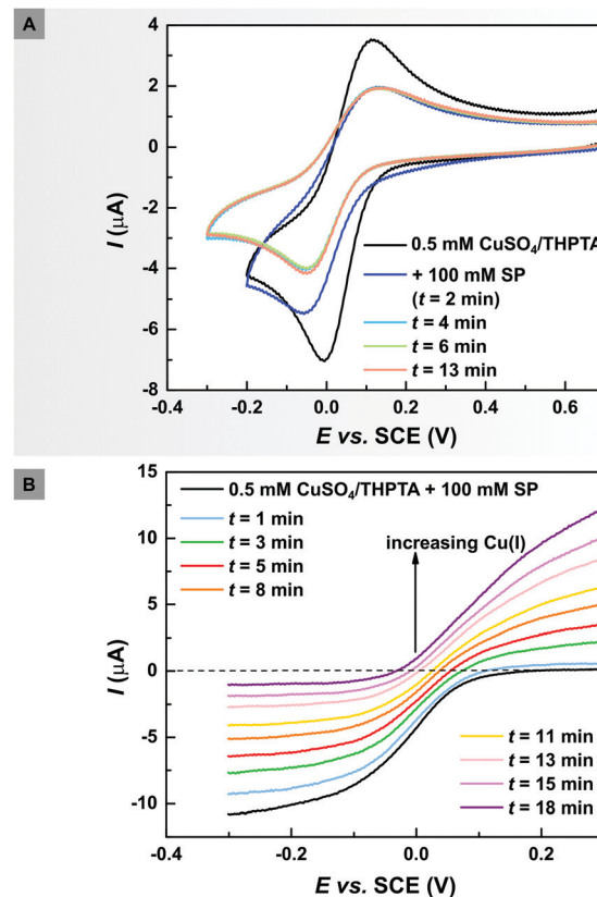
Fig. 4 (A) CVs of 0.5 mM Cu II SO 4 /THPTA in PBS, recorded on a glassy carbon (GC) working electrode at v = 0.2 \text{ V s}^{-1} , in the absence and presence of 100 mM SP. (B) LSV of 0.5 mM Cu II SO 4 /THPTA + 100 mM SP, in PBS, recorded on a GC working electrode at v = 0.01 \text{ V s}^{-1} under UV light (3.6 mW cm -2 ). The GC tip was attached to a rotating disk electrode (RDE), rotating at a speed of 2500 rpm.
