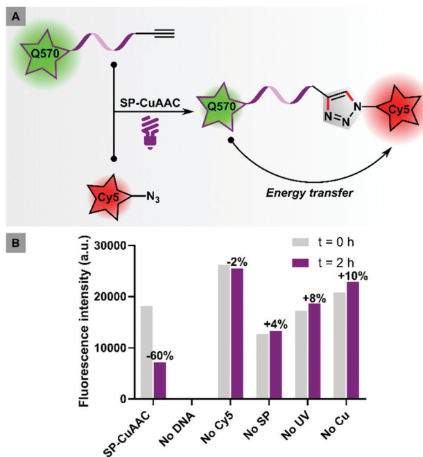
Fig. 2 SP -Mediated photoinduced CuAAC, reaction conditions: [Q570-DNA]/[ N_3 -Cy5]/[ CuSO_4 ]/[THPTA]/[ SP ]: 1/1.1/2.5/12.5/1000, [Q570-DNA] = 0.1 mM, in PBS with 3.7% DMSO at r.t., under UV light (6 mW cm -2 ) in an ambient atmosphere for 2 h. (A) Förster resonance energy transfer occurs upon SP -CuAAC. (B) Microplate reader measurement of the Q570 fluorescence intensity drop ( \lambda_{ex} = 548 nm, \lambda_{em} = 568 nm) due to FRET.
