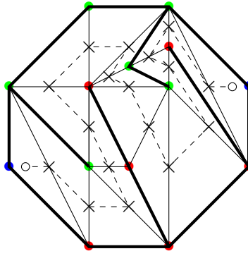
Figure 4: The graph associated to the complex of interior faces of the link from Figure 3.
