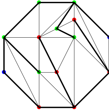
Figure 3: The link in some \Delta of a certain blue vertex on \mathbb{P}^n \times \mathbb{P}^m \times \mathbb{P}^\ell .
