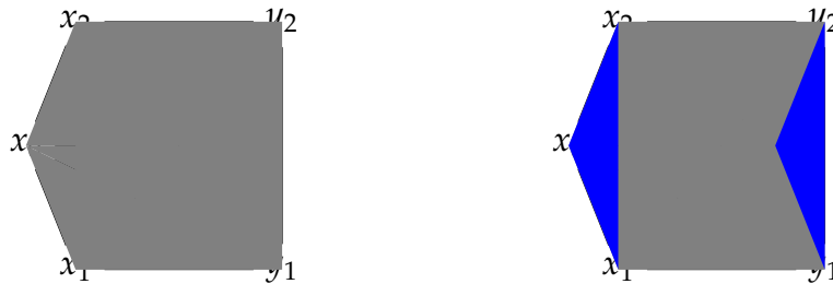
Figure 5: A cylindrical \Delta on \mathbb{P}^2 \times \mathbb{P}^2 , to which adding irrelevant faces produces a Cohen–Macaulay complex
