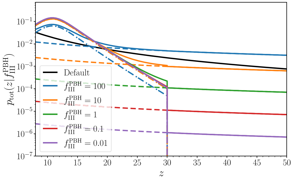
Figure 4. Prior based on the mixture model p_{\text{tot}} (solid lines), ranging from f_{\text{III}}^{\text{PBH}} = 100 (blue), 10 (orange), 1 (green), 0.1 (red), and 0.01 (purple). The dashed lines and dashed-dotted lines represent the individual contribution from PBH mergers and Population III BBH mergers (which are truncated at z_{\text{crit}} ), respectively.
