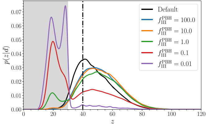
Figure 3. Posteriors of the system (M_{\text{tot}}, q, \iota, z) = (40M_{\odot}, 1, \pi/3, 40) , using p_{\text{tot}}(z) evaluated at f_{\text{III}}^{\text{PBH}} = 100 (blue), 10 (orange), 1 (green), 0.1 (red), and 0.01 (purple). The black solid line shows the default posterior. The black dashed line indicates z_{\text{true}} = 40 , and the gray area indicates the astrophysical region z < z_{\text{crit}} .
