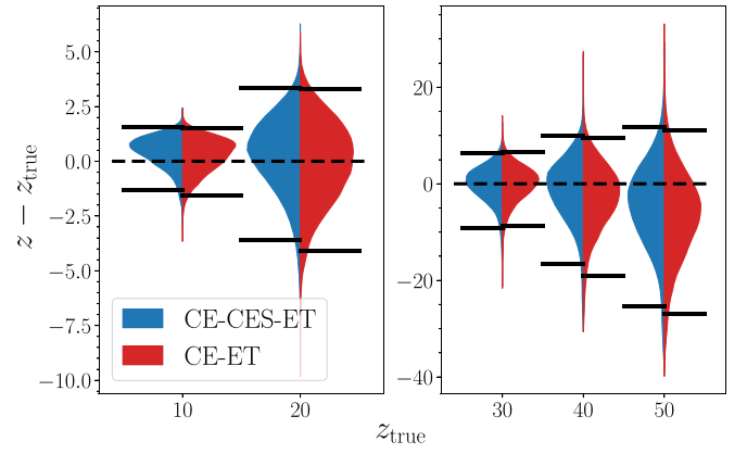
Figure 1. Redshift posteriors (offset by the true values) for sources with (M_{\text{tot}}, q, \iota) = (40 M_{\odot}, 1, \pi/6) at five different redshifts observed by CE–ET (red) and CE–CES–ET (blue). The solid horizontal lines show the 95% credible intervals, whereas the dashed lines mark z_{\text{true}} .
