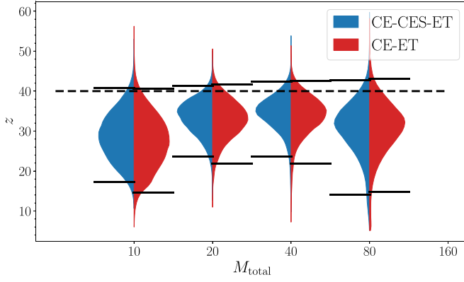
Figure 2. Redshift posteriors for sources with (q, \iota, z) = (1, 0, 40) at four different total masses observed by CE-ET (red) and CE-CES-ET (blue). The solid horizontal lines show the 95% credible intervals, whereas the dashed line marks z_{\text{true}} . Only sources with S/N \geq 12 are included.
