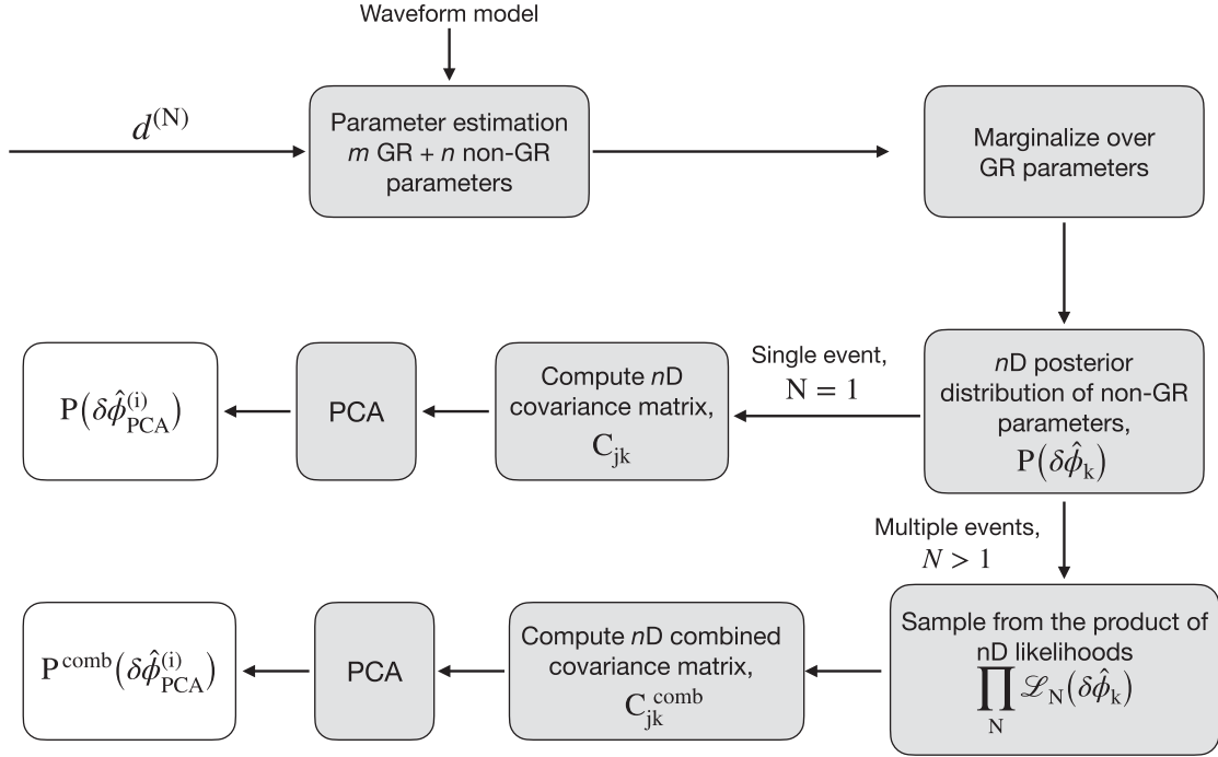
FIG. 1. Flowchart showing the hierarchy of steps followed to obtain the posterior distribution of PCA parameters, starting from the data, for n number of events. See the text for more details.
