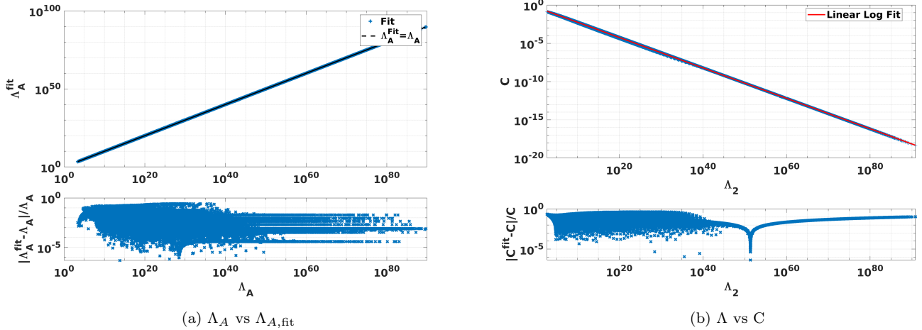
FIG. 5. DWD universal relations. The first panel shows that the binary Love relation, \Lambda_A = \Lambda_A(q, \Lambda_S) , is reasonably approximated by a functional form from the neutron star literature [46, 57, 60], using the new coefficients from Table I, whereas the second panel demonstrates that for DWDs \Lambda_2 can be well approximated by the fit given in Equation (24), effectively \Lambda_2 \propto C^{5.1} .
