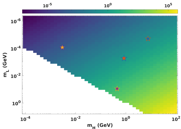
FIG. 3. Frequency at merger contact in Hz for two identical, maximum-mass dark white dwarfs as a function of m_H and m_L .
