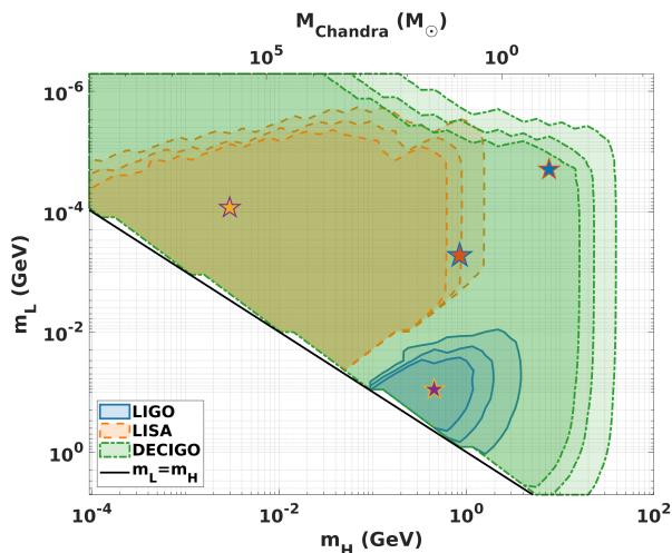
FIG. 4. Gravitational wave detectability (SNR) of identical, maximum-mass DWD mergers. Shaded regions correspond to \text{SNR} \geq 8 . SNR contours are derived from Eqs. ((18)) and ((19)) with a frequency cutoff of f_{\text{contact}} (Eq. (20)) and plotted at three luminosity distances, D_L = \{100, 250, 450\} Mpc (lighter to darker) using design sensitivity curves for LIGO, LISA and DECIGO [52–54]. Clearly, the different detectors will probe different regions of the parameter space in a complementary fashion and combined, LIGO and LISA will probe much of the m_L \sim 10^{-3} GeV, m_H \sim 10^{-4} GeV parameter space.
