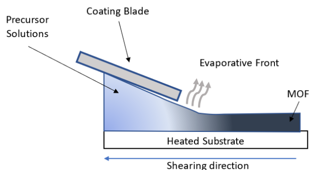
Figure 7: Schematic of the solution shearing method of fabrication and deposition of the thick MOF samples. The MOF self assembles at the leading edge of the shearing blade.
