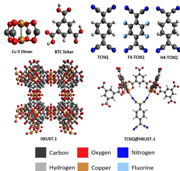
Figure 1: Schematic of the building blocks and guest molecules of the guest@HKUST-1 system: (top) Cu II dimer metal node (note that the Cu II paddle-wheel dimer shows the \text{Cu}^{2+} coordinated to eight oxygens from four separate BTC molecules), BTC linker, and the TCNQ, F 4 -TCNQ, and H 4 -TCNQ guest molecules. (Bottom) the full assembly of a single unit cell of the pristine HKUST-1 is shown along with a zoomed in representation of the TCNQ@HKUST-1 bonding environment as described by Allendorf et al. [3]
