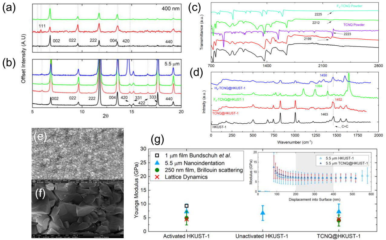
Figure 3: Characterization of samples. (a) XRD data for F_4 -TCNQ@HKUST-1 (green), TCNQ@HKUST-1 (red) and HKUST-1 (black) 400 nm thin films and (b) and XRD for the H_4 -TCNQ@HKUST-1 (blue), F_4 -TCNQ@HKUST-1 (green), TCNQ@HKUST-1 (red) and HKUST-1 (black) 5.5 \mu\text{m} thick MOF samples. We see little evidence of excess TCNQ, F_4 -TCNQ and H_4 -TCNQ that did not diffuse into the pores. (c) FTIR spectra for 5.5 \mu\text{m} thick pristine (black) TCNQ@HKUST-1 (red) and F_4 -TCNQ@HKUST-1 (green) MOFs compared to TCNQ (purple) and F_4 -TCNQ (aqua) molecules in powder form. The respective nitrile stretch is labeled in the spectra, the magnitude of the red shift occurring from the guest species in powder form to infiltrated form shows the degree that the TCNQ/ F_4 -TCNQ interacts with the coordination sites of the framework. (d) Raman spectra for the 5.5 \mu\text{m} thick pristine (black), TCNQ@HKUST-1 (red), F_4 -TCNQ@HKUST-1 (green) and H_4 -TCNQ@HKUST-1 (blue) MOFs. The C=C stretching frequency is labeled. The shift of the C=C stretching frequency upon infiltration and the additional peaks occurring between 1101 – 1343 \text{cm}^{-1} indicate the TCNQ and F_4 / H_4 -TCNQ derivatives coordinate to the \text{Cu}^{2+} ions in the framework. (e) Planar SEM images for the 400 nm pristine polycrystalline HKUST-1 SURMOF thin films fabricated by LBL-LPE from KIT and (f) 5.5 \mu\text{m} thick polycrystalline HKUST-1 samples fabricated using solution shearing at UVA. (g) Young's Modulus for 400 nm and 5.5 \mu\text{m} pristine and TCNQ@HKUST-1 samples measured by pump probe Brillouin scattering and nanoindentation respectively. The results are compared to the lattice dynamics derived Young's Modulus using a Poisson ratio of 0.49, and also to nanoindentation results for a 1 \mu\text{m} HKUST-1 film from Bundschuh et al. (46) The inset shows the full range of indenter displacement on the 5.5 \mu\text{m} pristine and TCNQ@HKUST-1 samples, however only data in the shaded region was used for analysis.
