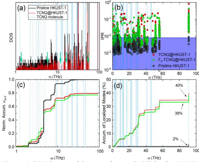
Figure 6: (a) Vibrational density of states (DOS) for the HKUST-1 (black) and TCNQ@HKUST-1 (red) compared to the vibrational spectrum of a single isolated TCNQ molecule (blue dotted lines). The DOS for F 4 -TCNQ@HKUST-1 has been left off for clarity. We see the emergence of new modes upon infiltration that overlap with the TCNQ molecular modes (pointed out by the green arrows). (b) Mode resolved inverse participation ratio (IPR) calculated at the \Gamma wave vector only. The blue shaded region corresponds to the delocalized modes, where the transition from delocalized to localized modes occurs at an \text{IPR} \geq 0.008 , corresponding to eigenvectors that are spread across 20% or less of the atoms in the supercell (125 atoms). (c) Thermal conductivity accumulation from non-propagating modes (diffusons) calculated from Allen-Feldman theory at 300 K normalized to the \kappa_{A-F} for pristine HKUST-1 and (d) the accumulation of IPR calculated localized modes at the \Gamma wave vector in pristine HKUST-1 (black), TCNQ@HKUST-1 (red), and F 4 -TCNQ@HKUST-1 (green), and an isolated TCNQ molecule (blue dotted lines).
