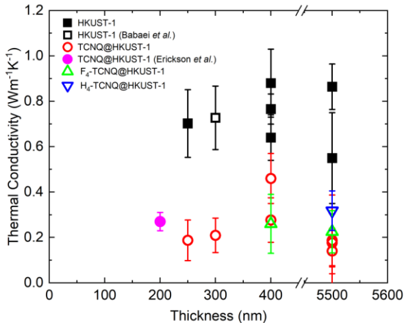
Figure 2: Experimentally measured thermal conductivity vs. thickness of activated pristine HKUST-1 (black filled squares) and infiltrated HKUST-1 (open symbols). The reported measured thermal conductivity of a 200 nm thick film of TCNQ@HKUST-1 (pink filled circle) from Erickson et al. (2) and a 300 nm pristine HKUST-1 film (black open square) from our previous work(13) are also shown for reference. Table S1 lists details on the individual samples.
