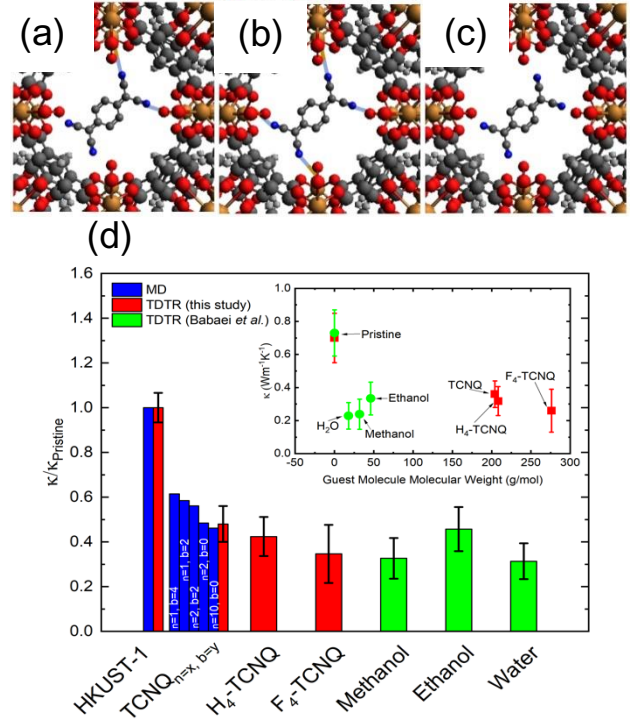
Figure 4: (a)-(c) Visualizations of the infiltrated pore bonding morphologies considered for MD simulations. The nomenclature 'TCNQ n=x,b=y @HKUST-1' indicates the adsorbed bonding conditions, where n is the number of TCNQ molecules per pore and b is the number of covalent bonds formed between the guest and host ( b=0 indicates unbound, free state). (a) Two covalent bonds on one side ( cis to each other) of a single TCNQ molecule ( n=1, b=2 ), (b) a single TCNQ creates four covalent bonds with the host ( n=1, b=4 ), and (c) single, unbonded "free state" TCNQ molecule ( n=1, b=0 ). The concentration of molecules within the pore is varied from one to ten. (d) Normalized room temperature thermal conductivity comparing the MD (blue) to the TDTR measured results for HKUST-1 and guest@HKUST-1 from this study (red) and our previous study (green).(13) All thermal conductivities have been normalized to the thermal conductivity of the pristine HKUST-1 ( \kappa_{\text{pristine}} ). We note the experimental data for the 400 nm thin films are shown for TCNQ and F 4 -TCNQ, while the H 4 -TCNQ results are from the 5.5 \mu\text{m} thick samples. The HKUST-1 infiltrated with methanol, ethanol and water were 200 nm thick and are from our previous work (green).(13) The inset shows the experimentally measured thermal conductivity for the guest molecules as a function of molecular weight.
