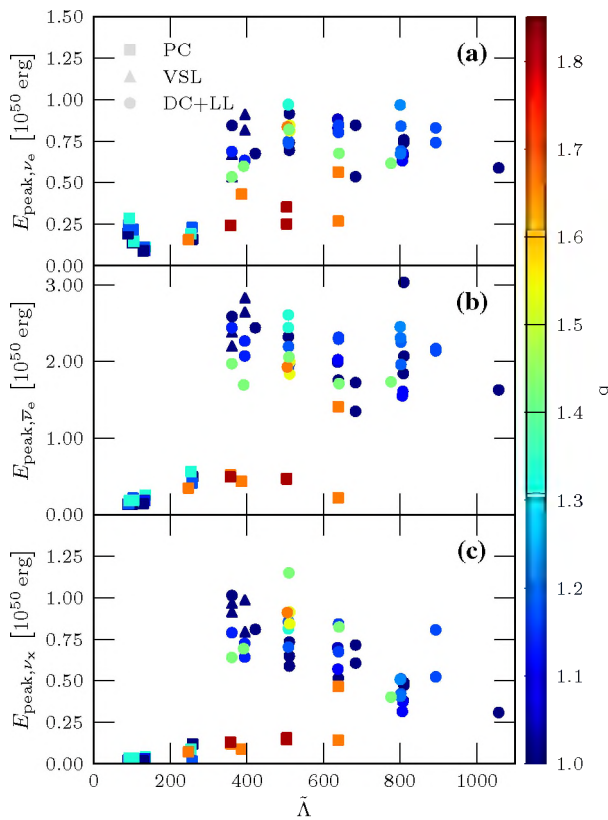
Fig. 4 Energy emitted by the peak E_{\text{peak}} as a function of the reduced dimensionless tidal parameter \tilde{A} for electron neutrinos (panel a), electron antineutrinos (b) and heavy lepton neutrinos (c). Colour indicates the BNS mass ratio
