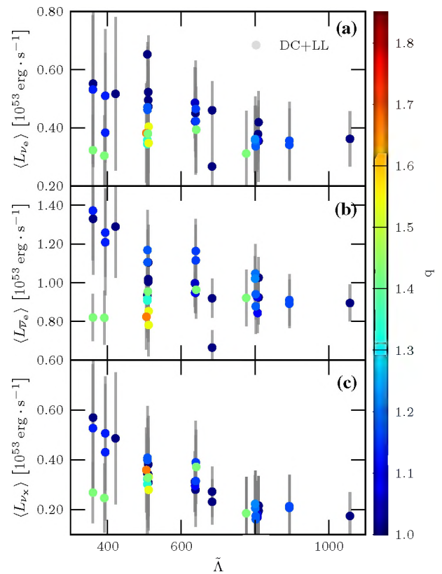
Fig. 5 Average luminosity \langle L_{\nu} \rangle as a function of the reduced dimensionless tidal deformability \tilde{A} for electron neutrinos (panel a), electron antineutrinos (b) and heavy lepton neutrinos (c) for DC and LL simulations. Colour indicates the BNS mass ratio while grey bars the standard deviation of the values
