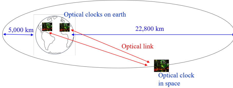
Figure 3. Schematic of the proposed mission to test Fundamental physics with an Optical Clock Orbiting in Space (FOCOS). A high-performance optical clock in an elliptical orbit around Earth is connected to ground optical clocks through a high stability optical link. Clock comparisons will enable tests of fundamental physics and provide an international clock reference for timing/geodetic applications.
