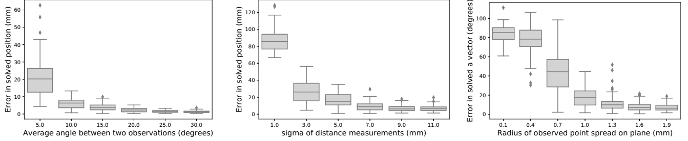
Fig. 5. Simulated experiments demonstrate no-rotation, same-distance, and no-spread degeneracy. For each type of degeneracy as described in Section III-D, error in the solved parameter (y axis) increases as the degenerate case is approached. However, relatively small deviations from each degenerate case dramatically reduce solution error. Each box represents 100 trials, each with 32 observations and Gaussian measurement noise ( \mu = 0\text{mm} , \sigma = 0.5\text{mm} ). Diamonds indicate outliers.
