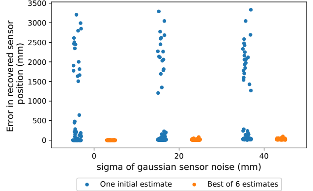
Fig. 4. Search of six initial estimates for optimization solver results in lower error in simulation. Blue points represent performing the optimization procedure with only one initial estimate for the free variables, while orange points represent picking the best of six initial estimates, based on loss. Solutions with a very high error rate are eliminated by search over initial estimates. 100 trials per column, 32 observations per trial.
