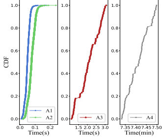
Fig. 8: Execution Time
