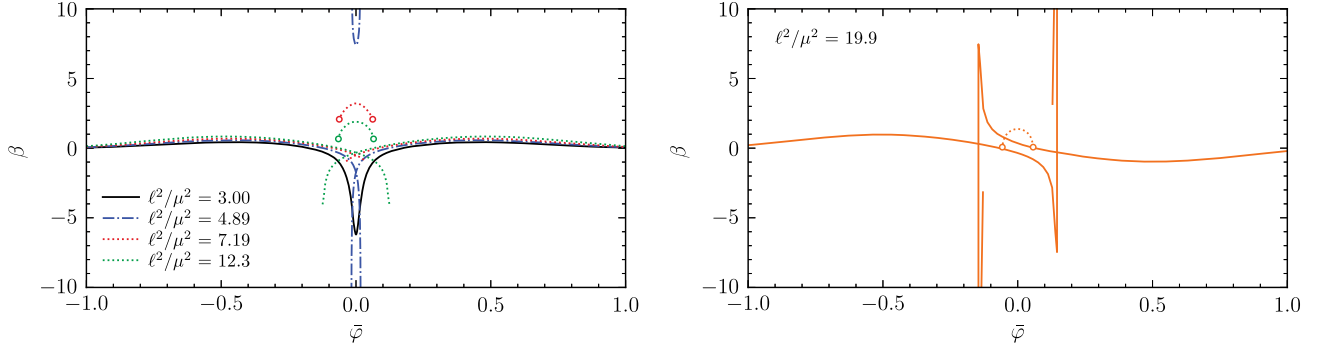
FIG. 11. Black hole sensitivities \beta in the Gaussian theory as functions of \bar{\varphi} and \ell/\mu . We consider the same constant entropy solutions as in Fig. 6. For values (\ell/\mu)^2 \lesssim 3.82 the curve includes a stable Schwarzschild solution at \bar{\varphi} = 0 , with \alpha = 0 , but \beta < 0 can be large, cf. (\ell/\mu)^2 = 3.00 . When (\ell/\mu)^2 \gtrsim 3.82 the curve is multivalued. The segments bracketed by the circles denote the “Schwarzschild branches” with \beta > 0 . They include an unstable Schwarzschild solution at \bar{\varphi} = 0 , with \alpha = 0 . The remainder of the curves form two “scalarized branches” that include the stable scalarized black holes with \bar{\varphi} = 0 and \alpha \neq 0 . For (\ell/\mu)^2 \in [3.82, 5.61] , the three branches are connected. At their junction, M/\mu features a cusp, cf. Fig. 6, and the slope of \alpha , that is \beta here, is infinite. When (\ell/\mu)^2 \gtrsim 5.61 , the branches are discontinuous due to the violation of the horizon bound (45). But when (\ell/\mu)^2 \in [13.6, 13.8] and (\ell/\mu)^2 \gtrsim 14.0 , the ratio M/\mu of scalarized branches also features a cusp and \beta hence diverges. This is illustrated with (\ell/\mu)^2 = 19.9 in the right panel.
