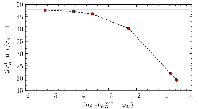
FIG. 3. Numerical Gauss-Bonnet scalar \mathcal{G} r_H^4 evaluated at the event horizon r_* = r/r_H = 1 for a sequence of black holes with constant (\ell/\mu)^2 = 10^{-1} . As the scalar field at the horizon \varphi_H approaches its maximum allowed value \varphi_H^{\max} \approx 3.77526 , the Gauss-Bonnet scalar tends to the limit \mathcal{G} r_H^4 = 48 (horizontal line) predicted analytically by Eq. (18a).
