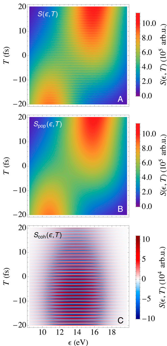
Fig. 6. TRPES signal for a 20-eV probe pulse of duration \tau = 200 as. The signal is shown for time delays around T = 0 fs. (A) The total signal S(\epsilon, T) and contributions from (B) populations S_{\text{pop}}(\epsilon, T) (Eq. 15) and (C) coherences S_{\text{coh}}(\epsilon, T) (Eq. 16) are exhibited.
