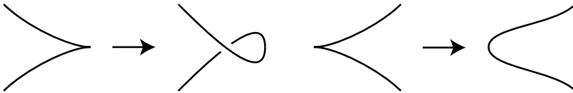
FIGURE 3. Resolution: changing a front projection of a Legendrian knot to a Lagrangian projection.
