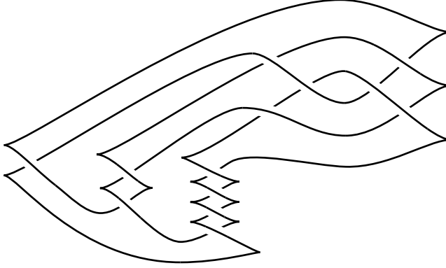
FIGURE 17. A knot that can be distinguished from its Legendrian mirror by the product on linearized cohomology.
