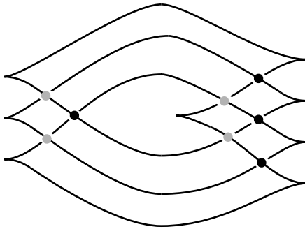
FIGURE 20. A Legendrian knot of type T(3, -4) .
