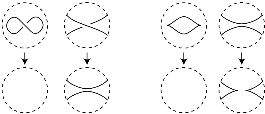
FIGURE 23. Two local moves representing exact Lagrangian cobordisms: the left two figures in each group are unknot filling; the right two figures are a pinch move. The left most group shows the Lagrangian projections and the right most group shows the front projections. (Arrows indicate going from the top of the cobordism towards the bottom.) For the pinch move in the Lagrangian projection, it is crucial that the crossing being resolved is contractible.
