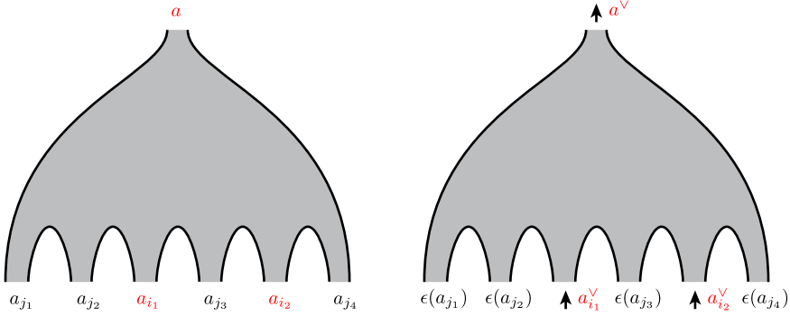
FIGURE 16. A disk with positive end at a and negative ends including a_{i_1} and a_{i_2} contributes an a^\vee term to m_2(a_{i_2}^\vee, a_{i_1}^\vee) .
