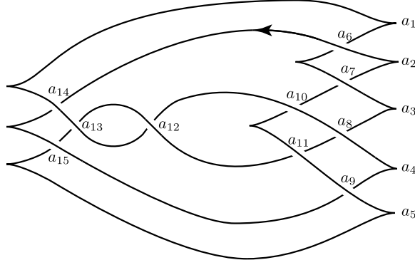
FIGURE 27. A Legendrian knot of type P(3, -3, -4) = m(10_{140}) . Crossings and right cusps (corresponding to Reeb chords for the resolution of this front) are labeled. A base point is placed in the loop at a_5 produced by the resolution.
