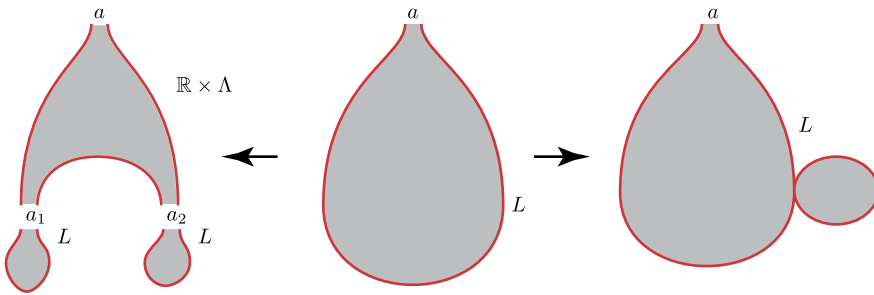
FIGURE 24. Possible degenerations of disks in \mathcal{M}^1(a) (the right one is actually forbidden).
