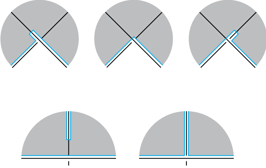
FIGURE 9. The new types of disks in \hat{\Delta}(a; b_1, \dots, b_n) . Along the top row we see a disk with a branch point on the right and left, and in the center we see a non-convex corner; the result is that a disk with such a non-convex corner is in the interior of a moduli space of dimension larger than 0. On the bottom row we see a disk with a branch point moving toward the boundary of the disk, at which point it limits to the union of two disks.
