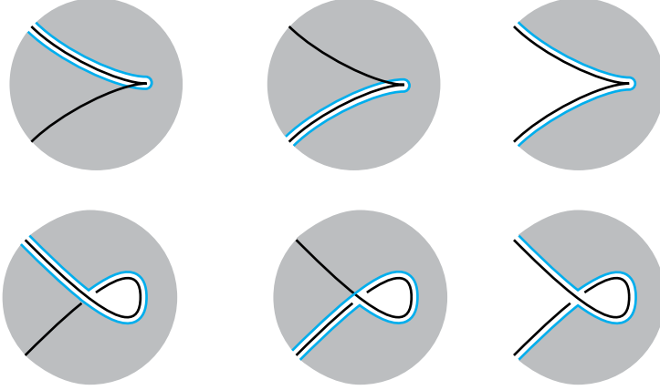
FIGURE 12. The top row shows the local picture of the image of u near a right cusp b . The bottom row shows the corresponding immersion in the Lagrangian projection. In the left and middle figures the contribution c(b) is b while in the right figure the contribution is b^2 . The image of the boundary of the disk is slightly offset for the sake of visibility.
