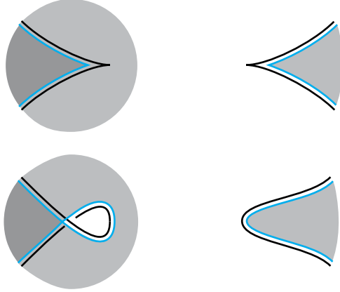
FIGURE 11. Top row are cusps in the front projection and the local image of the immersion u near the cusp point (darker shading indicates the map is locally two to one). The bottom row is the image of a corresponding immersion in the Lagrangian projection. The image of the boundary of the disk is slightly offset for the sake of visibility.
