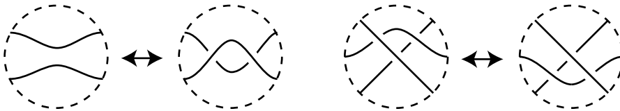
FIGURE 2. Reidemeister moves in the Lagrangian projection. On the left is the double point move and on the right is the triple point move. (These diagrams can be arbitrarily rotated or reflected.)
