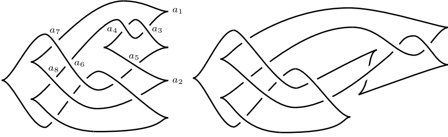
FIGURE 13. Two Legendrian representatives of the knot m(10_{132}) with maximal Thurston–Bennequin invariant. The one of the left has trivial contact homology and the one on the right has non-trivial contact homology.
