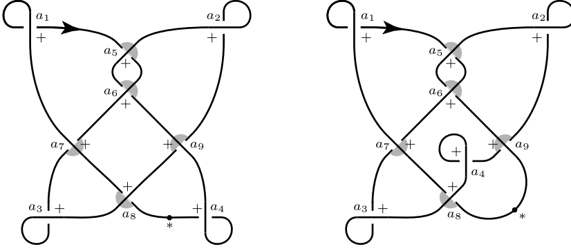
FIGURE 7. The Lagrangian projection of the two Chekanov knots. On the left is \Lambda_1 and on the right is \Lambda_2 . For each of the double points, the Reeb sign of one of the quadrants is shown, and quadrants with negative orientation signs are shaded.
