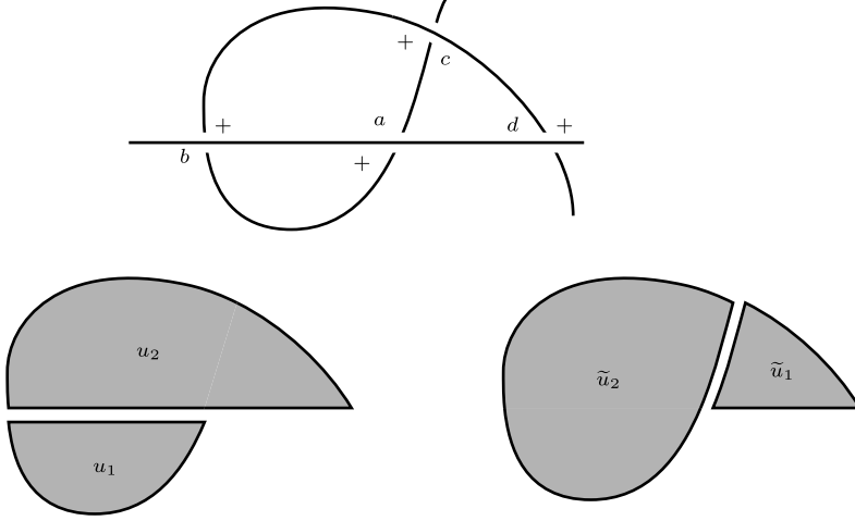
FIGURE 10. The top diagram is a portion of some Lagrangian projection \Pi(\Lambda) . On the bottom are disks contributing to \partial_\Lambda a . On the left we see u_1 contributes b to \partial_\Lambda a , while u_2 contributes d to \partial_\Lambda^2 a . On the right \tilde{u}_1 contributes dc to \partial_\Lambda a while \tilde{u}_2 shows the differential of dc has a term d in it. The two resulting d terms in \partial_\Lambda^2 a cancel.
