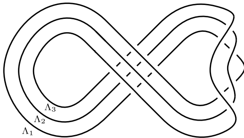
FIGURE 21. A 3-copy of the Legendrian unknot, in the xy projection. The perturbing Morse function on the unknot that yields this 3-copy has two critical points, a maximum in the upper right of the figure eight and a minimum in the lower right. This yields two triple points in the xy projection, which have further been perturbed to give two sets of 3 crossings as shown.
