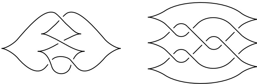
FIGURE 25. Two Legendrian knots with augmentations that do not come from fillings: the figure eight (left) and a knot of type m(8_{21}) (right).
