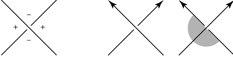
FIGURE 4. On the left we see the Reeb chord signs for each quadrant. On the right we see the orientation signs, which are - in the shaded quadrants and + in the other quadrants. The orientation signs depend on whether the crossing is positive (right) or negative (left).
