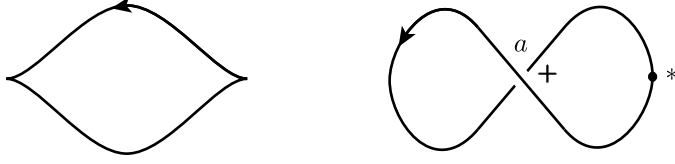
FIGURE 5. The standard Legendrian unknot \Lambda , in the front (left) and Lagrangian (right) projections. On the right, we have added a base point, and drawn the Reeb signs at the unique double point a ; because a is a negative crossing, all orientation signs are + .
