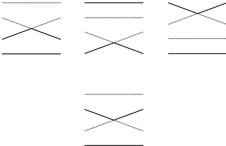
FIGURE 18. Top row shows allowable switches. The bottom row shows a disallowed switch. In each case the solid arcs are paired by the ruling, as are the dotted arcs.
