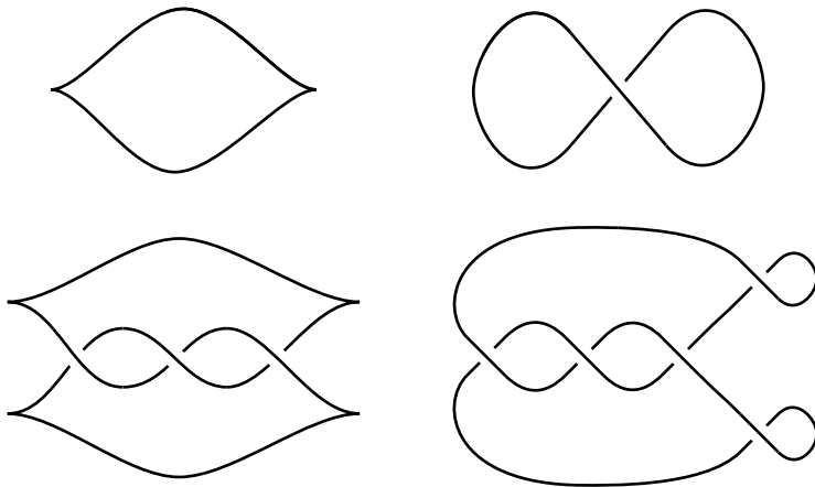
FIGURE 1. On the left are examples of the front projection of the unknot and the right handed trefoil knot. On the right are examples of the Lagrangian projection of the same knots; cf. Lemma 2.1.
