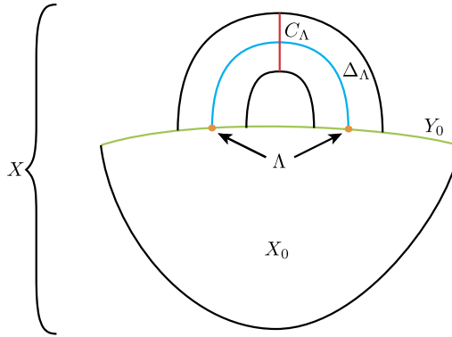
FIGURE 26. Attaching a critical Weinstein handle to a subcritical Weinstein domain X_0 along a Legendrian sphere \Lambda \subset Y_0 = \partial X_0 to produce a Weinstein domain X . Also pictured are the Lagrangian core \Delta_\Lambda and cocore C_\Lambda of the handle.
