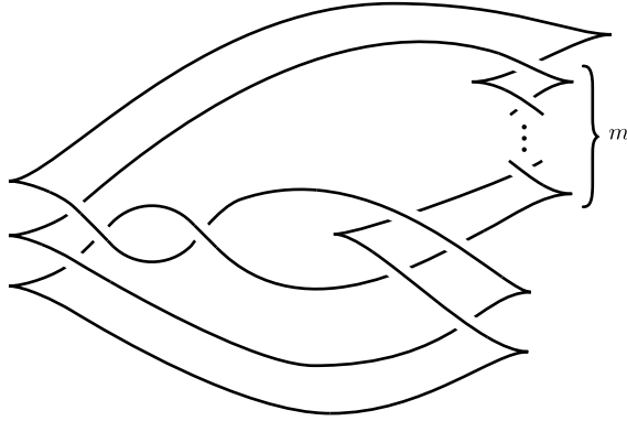
FIGURE 14. Legendrian representative of the pretzel knot P(3, -3, -3 - m) whose DGA is stable tame isomorphic to the DGA of the standard unknot.
