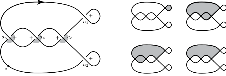
FIGURE 6. The Lagrangian projection of a Legendrian trefoil knot \Lambda is shown on the left. For each of the double points, the Reeb sign of one of the quadrants is shown (from which the others are easily deduced), and orientation signs are indicated by the shaded quadrants. On the right, the disks that go into the computation of \partial_\Lambda a_1 .
