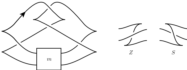
FIGURE 15. A Legendrian twist knot. The box is replaced with a tangle formed by concatenating m of the Z and S tangles shown on the right, in any order.
