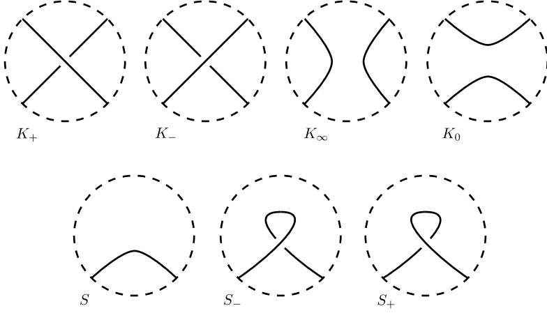
FIGURE 19. Diagram regions for the skein relations for F_K(a, z) .
