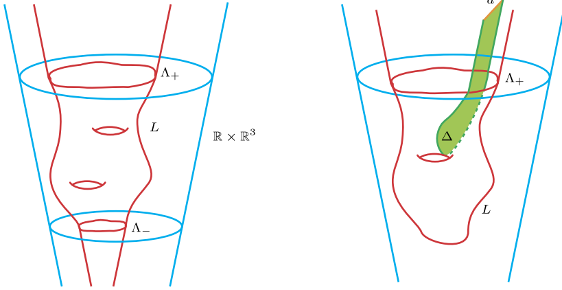
FIGURE 22. On the left, a Lagrangian cobordism from \Lambda_- to \Lambda_+ . On the right, a disk contributing to the augmentation \epsilon_L induced by a filling L of \Lambda_+ .
