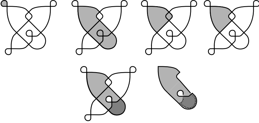
FIGURE 8. The five disks that go into the computation of \partial_{\Lambda} a_1 for the Chekanov example knot \Lambda_2 from Figure 7. The disk on the left of the bottom row is immersed, and the darker shaded part indicates where the immersion is two-to-one. The final picture on the bottom row is another view of this immersed disk: the boundary of the disk is slightly offset where the immersion is two-to-one to better indicate the overlapping region.
