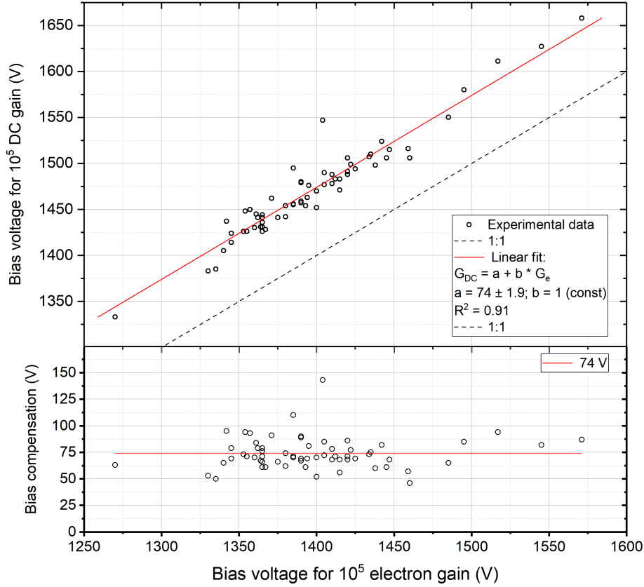
Figure 7. (Top) Bias voltage required for 10^5 electron gain as determined experimentally and for the same DC gain as listed in the specs. The 1 : 1 line reflects the distribution expected for the case of 100% collection efficiency. (Bottom) Difference between bias voltage for 10^5 DC gain and electron gain as a function of the latter.
