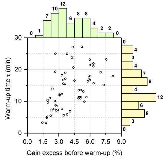
Figure 10. Distribution of the warm-up parameters for Planacon MCP-PMTs with the MCP stack resistance range 11–22 MΩ.
