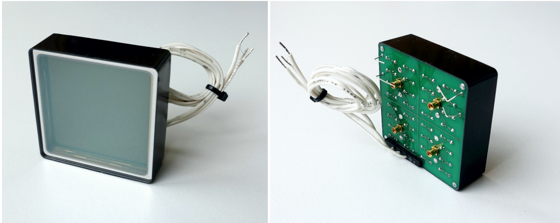
Figure 1. Front and back photos of Planacon XP85002/FIT-Q MCP-PMT as received from the factory. Dimensions of the sensor are 59 \times 59 \times 25\text{ mm}^3 , sensitive area of a single channel — 26.5 \times 26.5\text{ mm}^2 .
