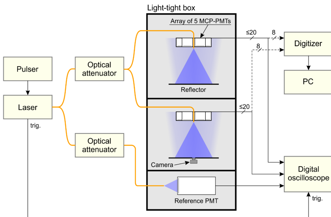
Figure 2. Simplified schematic diagram of the test bench.
