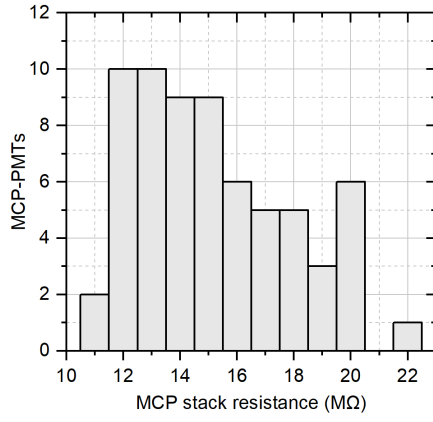
Figure 9. Stabilized MCP stack resistance of XP85002/FIT-Q Planacons measured after the warm-up.
