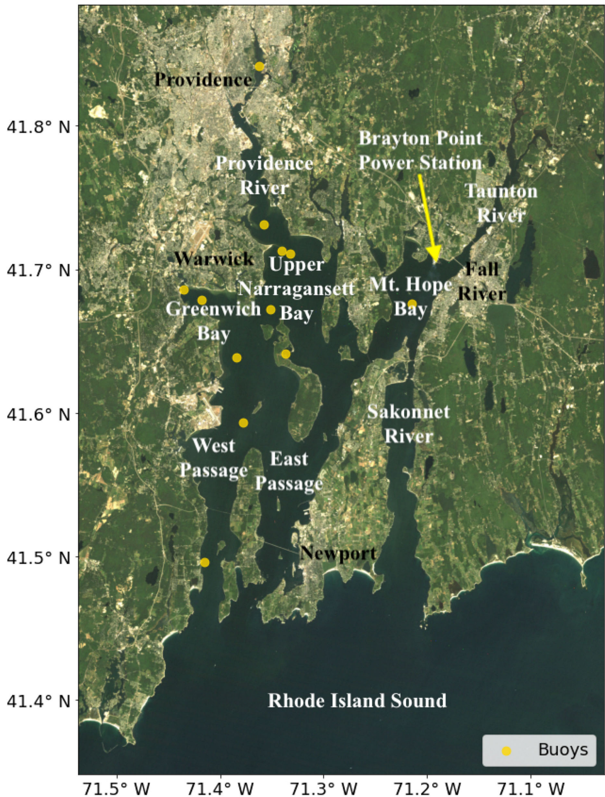
FIGURE 1 | Narragansett Bay shown in true color by a Landsat 5 scene on September 7th, 1984 with labeled regions and buoy locations. A plume of atmospheric discharge is faintly visible traveling southward from the Brayton Point Power Station.
