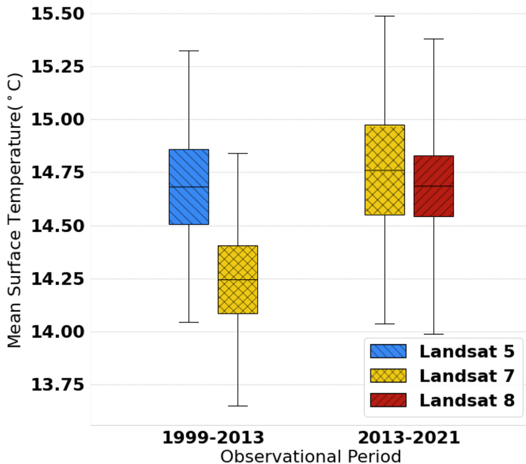
FIGURE 3 | Assessment of inter-satellite calibration by comparing surface temperature averaged over all of Narragansett Bay for overlapping time periods of each satellite. The central bars represent the means while the box edges represent propagated measurement uncertainty (from Table 1 ) and the whiskers represent sampling uncertainty estimated by bootstrapping.
