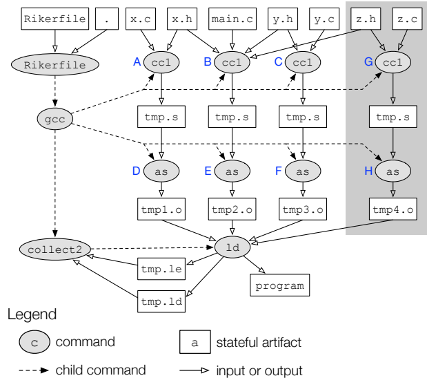
Figure 1: A dependency graph for the running example. Dashed edges show commands launching child commands, and solid edges indicate inputs and outputs. The grey box contains the modification induced by adding z.h and z.c to the build in Scenario 2 .
