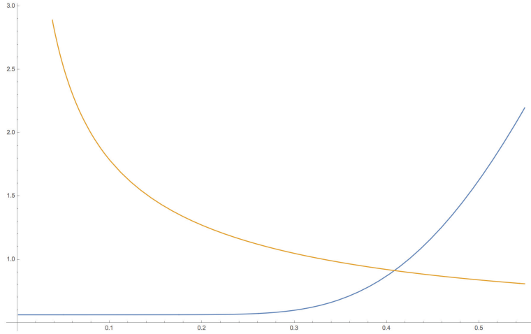
Figure 1. Plot of H(r) and \sqrt{r}C(r) on (0, \bar{\varepsilon}_2] .
