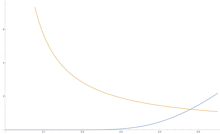
Figure 2. Plot of 2F(r) and C(r) on (0, \bar{\varepsilon}_2] .
