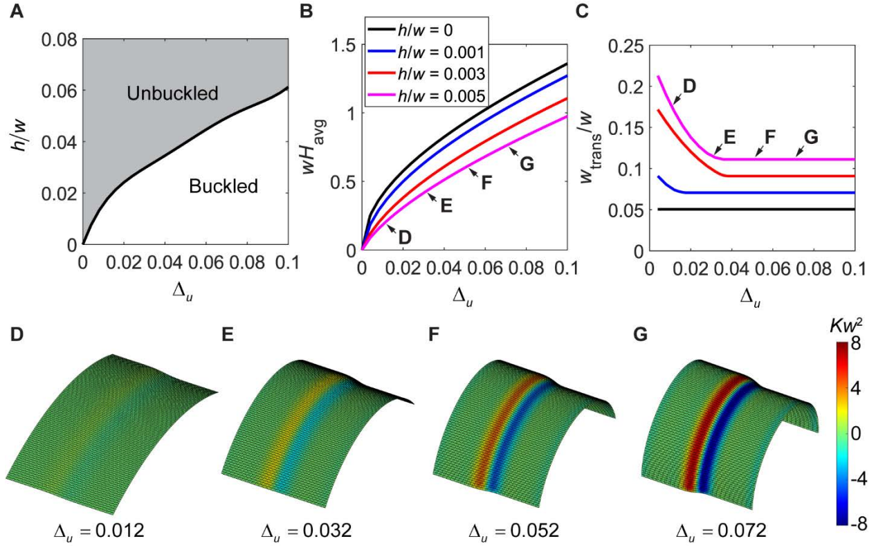
Fig. 6. The Effect of the stretch mismatch \Delta_u on the rolled shapes when \rho = 0.5 and \delta/w = 0.02 . (A) The dependence of the normalized critical thickness h_{\text{cr}}/w on \Delta_u (black solid line). The gray region ( h/w > h_{\text{cr}}/w ) indicates unbuckled configurations, whereas the white region ( h/w < h_{\text{cr}}/w ) indicates buckled configurations. (B and C) The influence of \Delta_u on the normalized average mean curvature wH_{\text{avg}} (B) and the width of the transitional bottle neck region w_{\text{trans}}/w (C) when h/w = 0 (isometric immersion in black), 0.001 (blue), 0.003 (red), and 0.005 (magenta). (D-G) The rolled shapes obtained from the theory for different \Delta_u when h/w = 0.005 .
