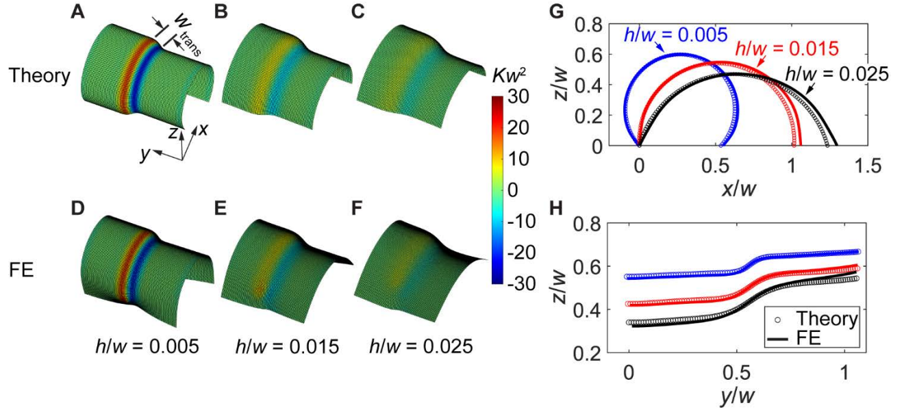
Fig. 3. Quantitative comparison between the theory and FE simulations. (A-F) The rolled shapes obtained from the theory (A-C) and FE simulations (D-F) for LCE bistris with the director parallel to the interface between the high- and low-temperature regions and of normalized thickness h/w = 0.005 (A and D), 0.015 (B and E), and 0.025 (C and F). (G and H) The profiles of the cross-section along (G) and perpendicular to (H) the interface between the two strips. The circular dots represent analytical results, whereas the solid lines represent the results from FE simulations. The blue, red, and black colors denote h/w = 0.005 , 0.015 , and 0.025 , respectively.
