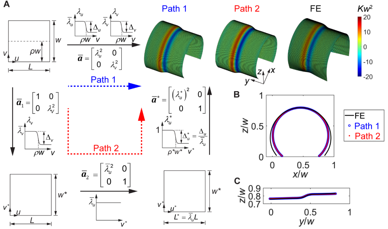
Fig. 5. Conversion from a prescribed metric tensor \bar{a} in LCE bistrisps with initial director either parallel or perpendicular to the interface into a unified metric tensor \bar{a}^* embedded to a bistrisp with modified geometry. (A) Shape morphing of a bistrisp subjected to \bar{a} (Path 1) is equivalent to that of the bistrisp with modified geometry subjected to \bar{a}^* (Path 2). The rolled shapes predicted by the analytical model following Path 1 and 2 and the FE simulation agree well. The profiles of the cross-section along (B) and perpendicular to (C) the interface between the high- and low-temperature strips based on Path 1 and 2 match perfectly.
