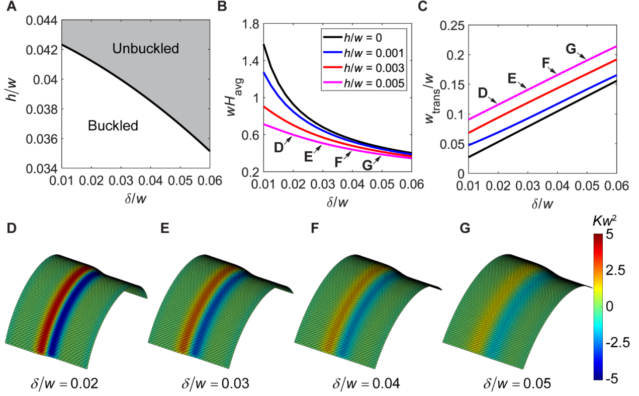
Fig. 7. The Effect of \delta on the rolled shapes when \rho = 0.5 and \Delta_u = 0.05 . (A) The dependence of h_{\text{cr}}/w on \delta (black solid line). The gray region ( h/w > h_{\text{cr}}/w ) indicates unbuckled configurations, whereas the white region ( h/w < h_{\text{cr}}/w ) indicates buckled configurations. (B and C) The influence of \delta on wH_{\text{avg}} (B) and w_{\text{trans}}/w (C) when h/w = 0 (isometric immersion in black), 0.001 (blue), 0.003 (red), and 0.005 (magenta). (D-G) The rolled shapes obtained from the theory for different \delta when h/w = 0.005 .
