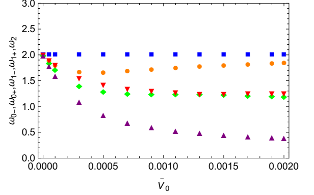
b. N = 10^4 fermions.
