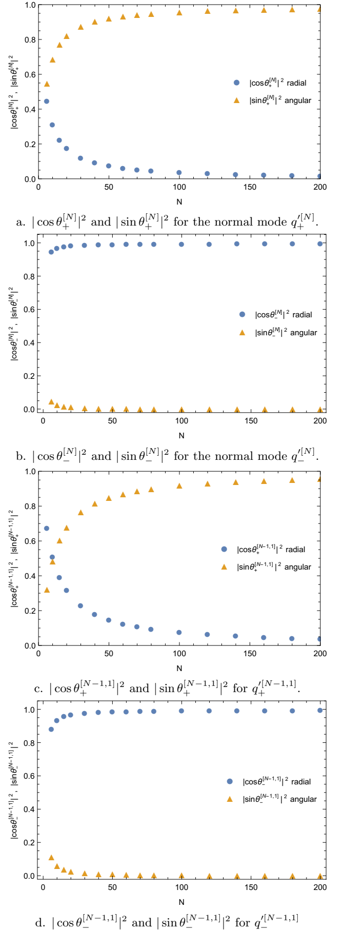
FIG. 1: The square of the mixing coefficients as a function of N for the weakly interacting BCS regime.
