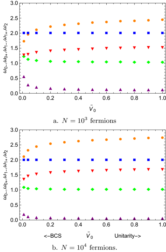
FIG. 5: Expanded view of Figs. (2a) and (2b) as unitarity is approached showing the stability of the angular frequencies \bar{\omega}_{0+} , \bar{\omega}_{1+} and \bar{\omega}_2 , and the gradual change of the radial frequencies \bar{\omega}_{0-} and \bar{\omega}_{1-} . ( \omega_{0-} orange dots; \omega_{0+} blue squares; \omega_{1-} red 'down' triangles; \omega_{1+} green diamonds; \omega_2 purple 'up' triangles).
