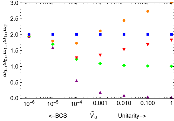
c. N = 10^5 fermions.
