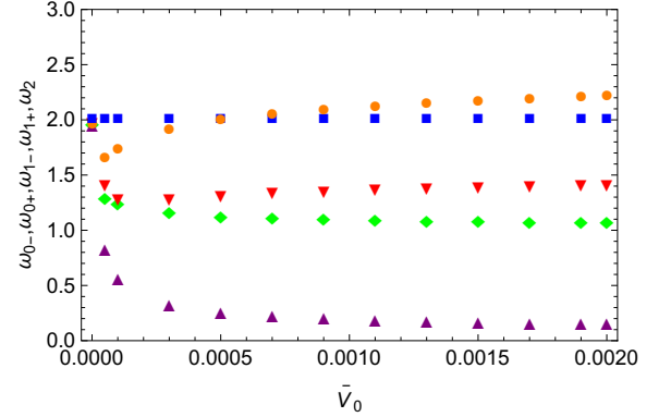
c. N = 10^5 fermions.
