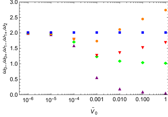
b. N = 10^4 fermions.
