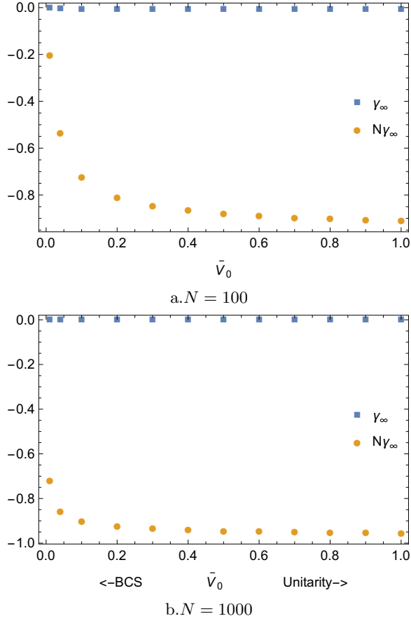
FIG. 6: Limits of \gamma_\infty and N\gamma_\infty as a function of \bar{V}_0 .
