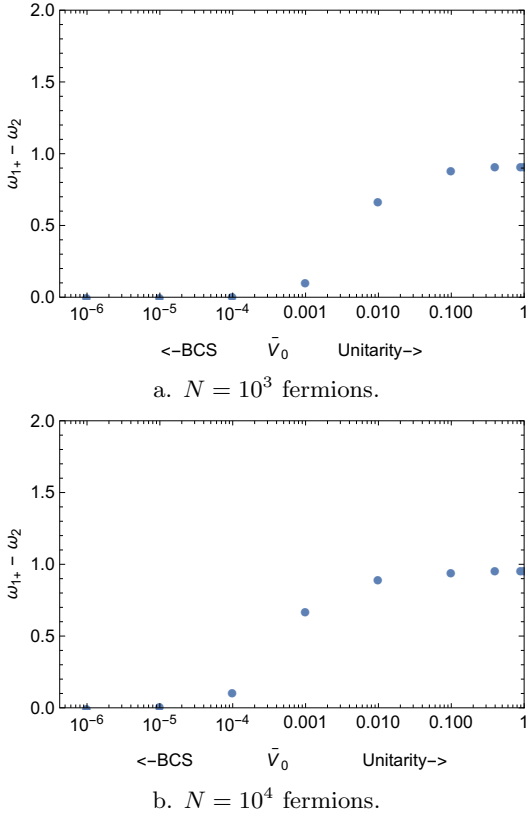
FIG. 4: Excitation gap in units of the trap frequency from the lowest two normal mode frequencies as a function of the interparticle interaction strength, \bar{V}_0 , from BCS to unitarity.
